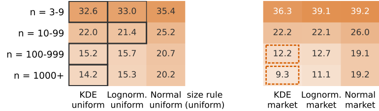
(c) Which one is closest inverts with dataset size
