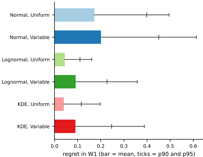
Synthetic arm, against its own target
