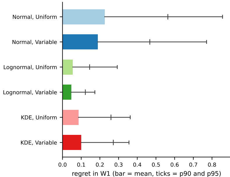
Empirical arm, cross-validated
