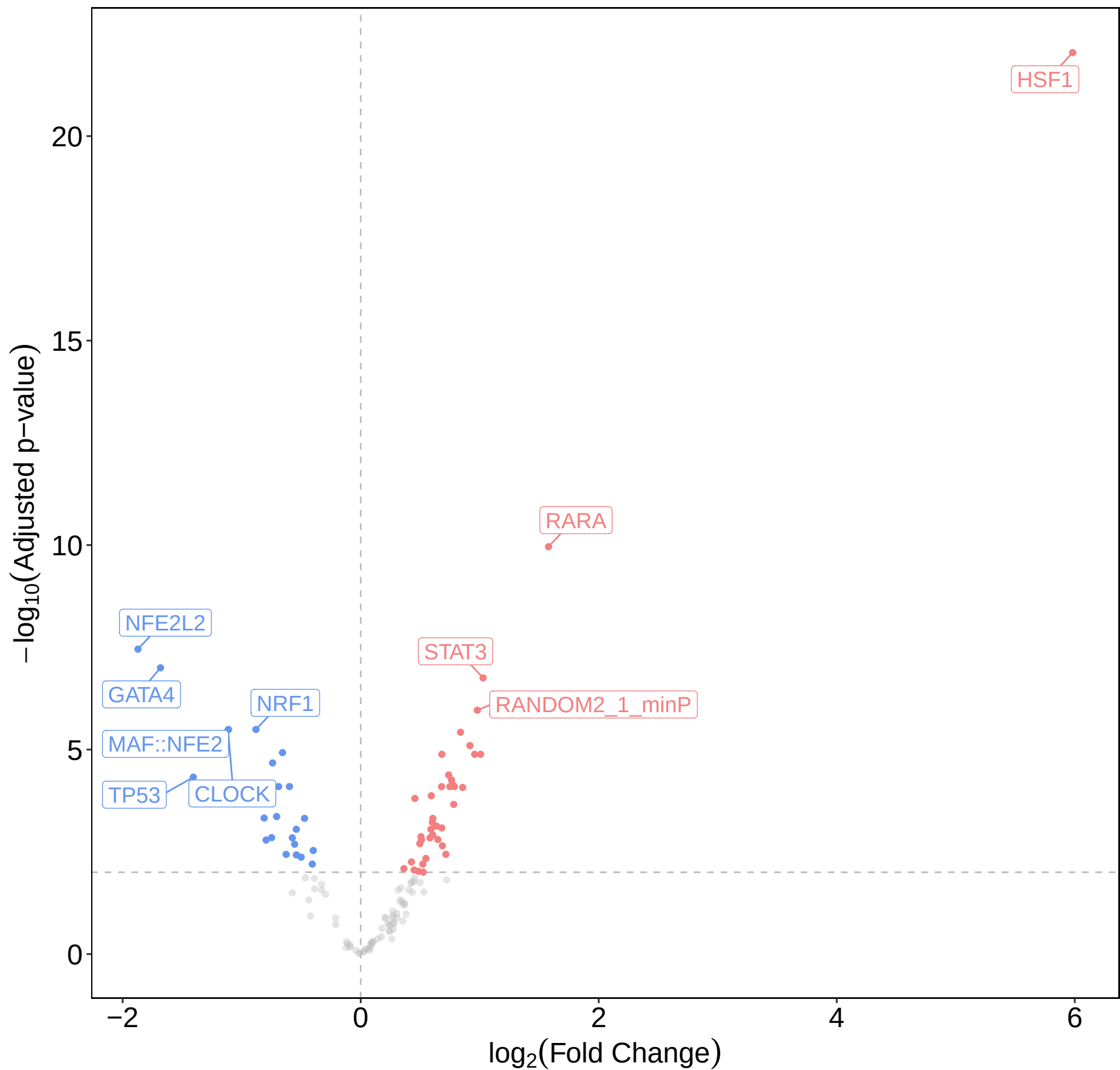
Heat vs. DMSO (p.adjusted \leq 0.01 )
