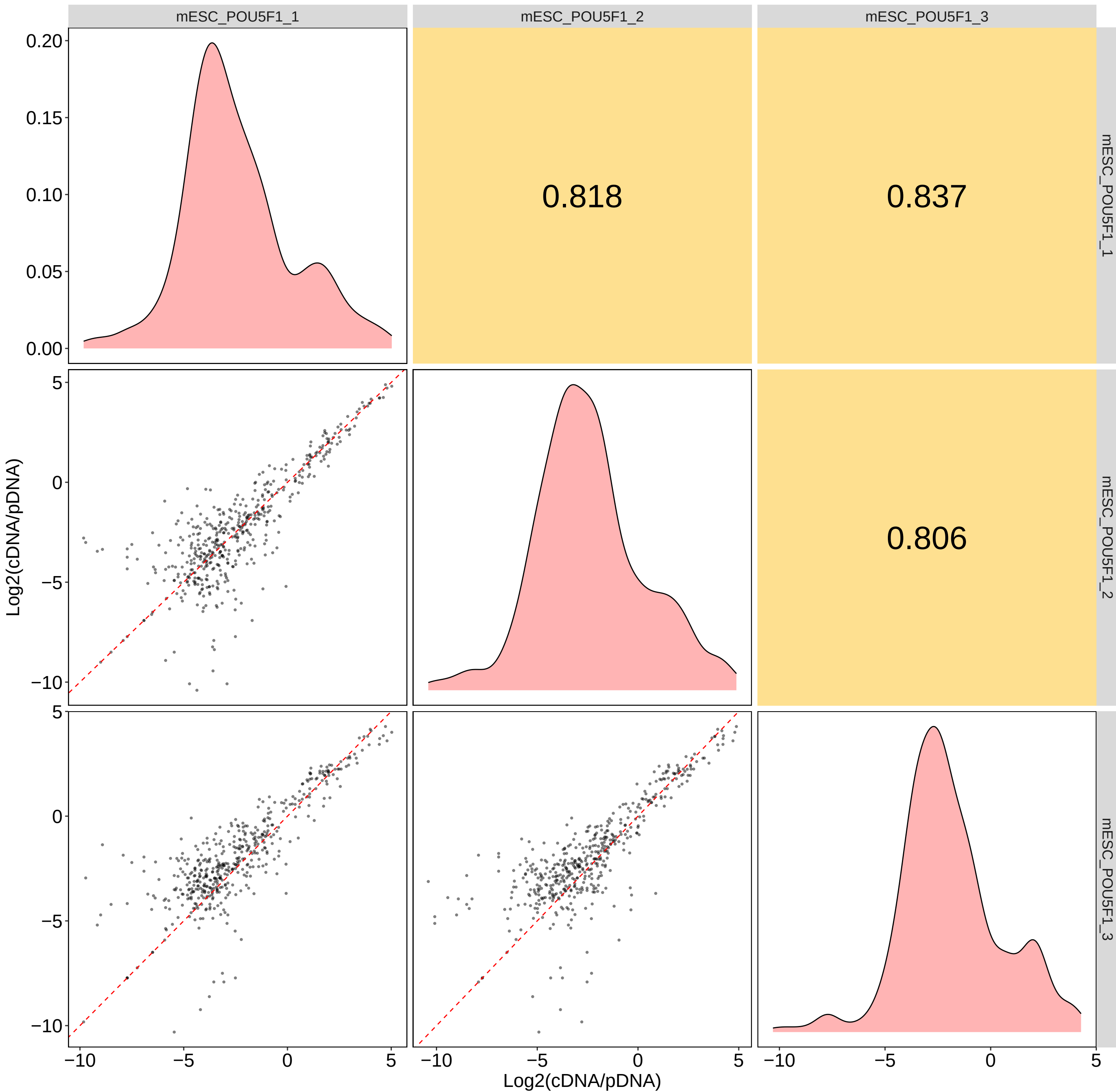
Replicate correlation of mESC_POU5F1
