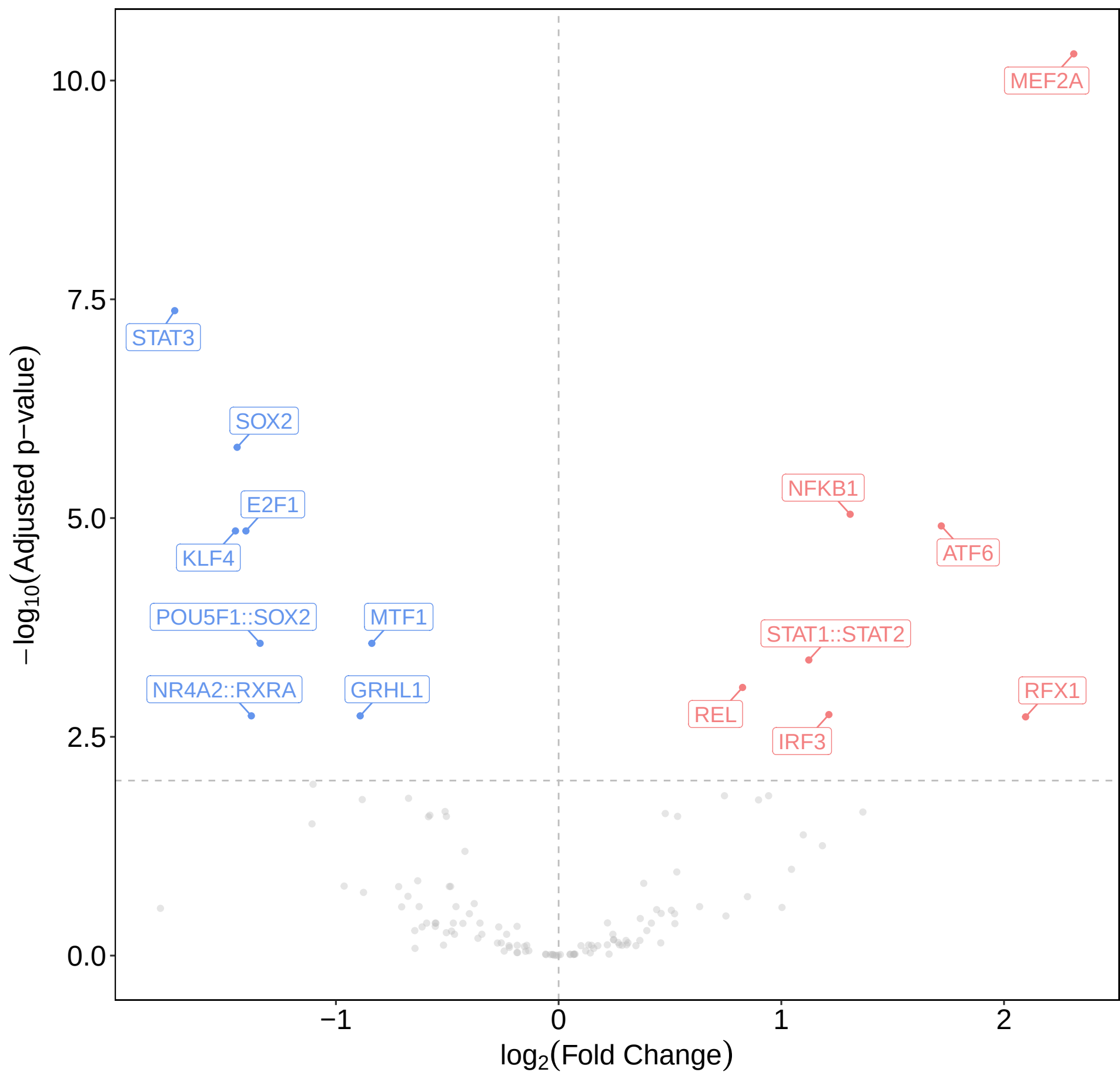
POU5F1 vs. DMSO (p.adjusted <= 0.01 )
