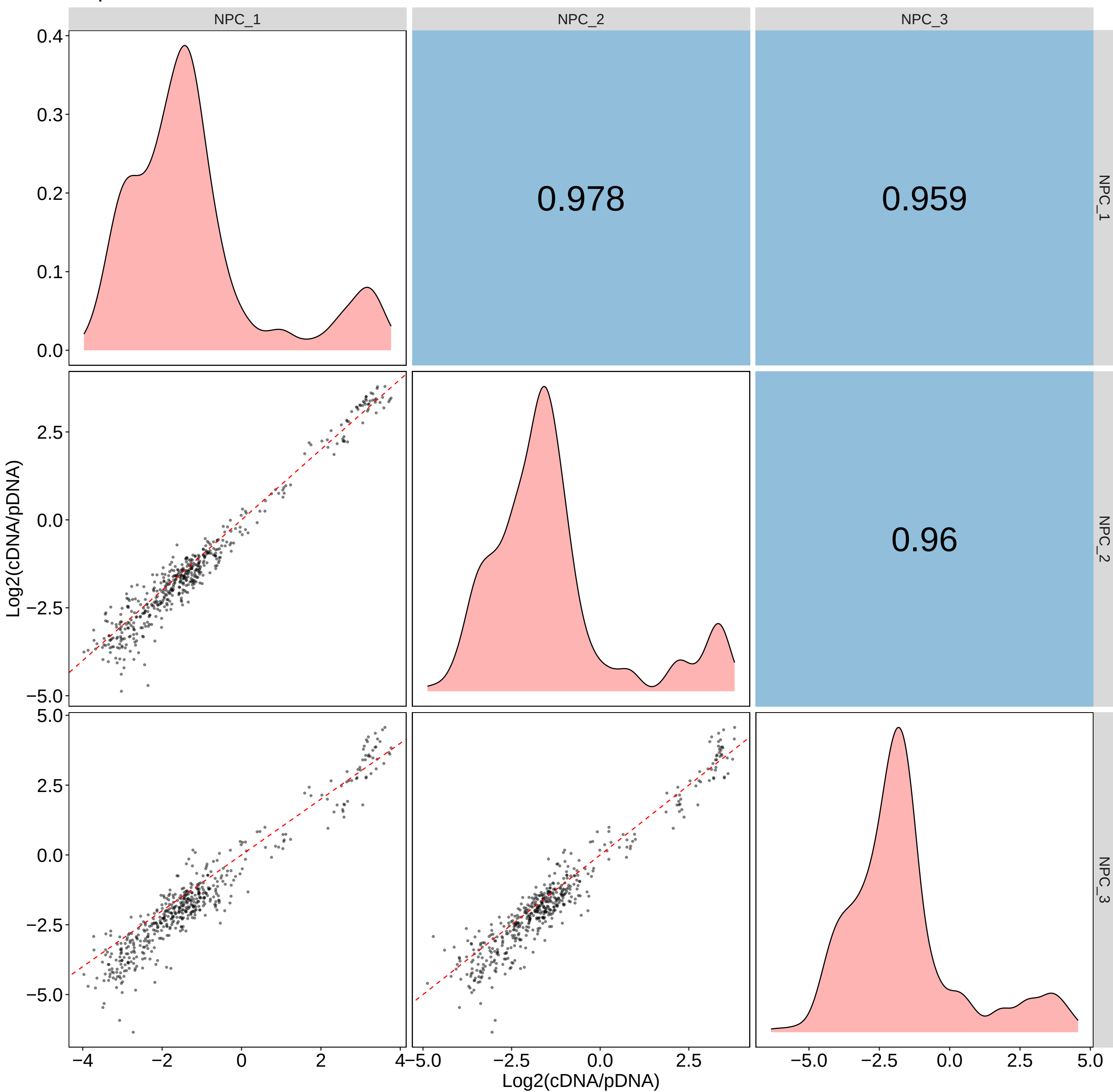
Replicate correlation of NPC
