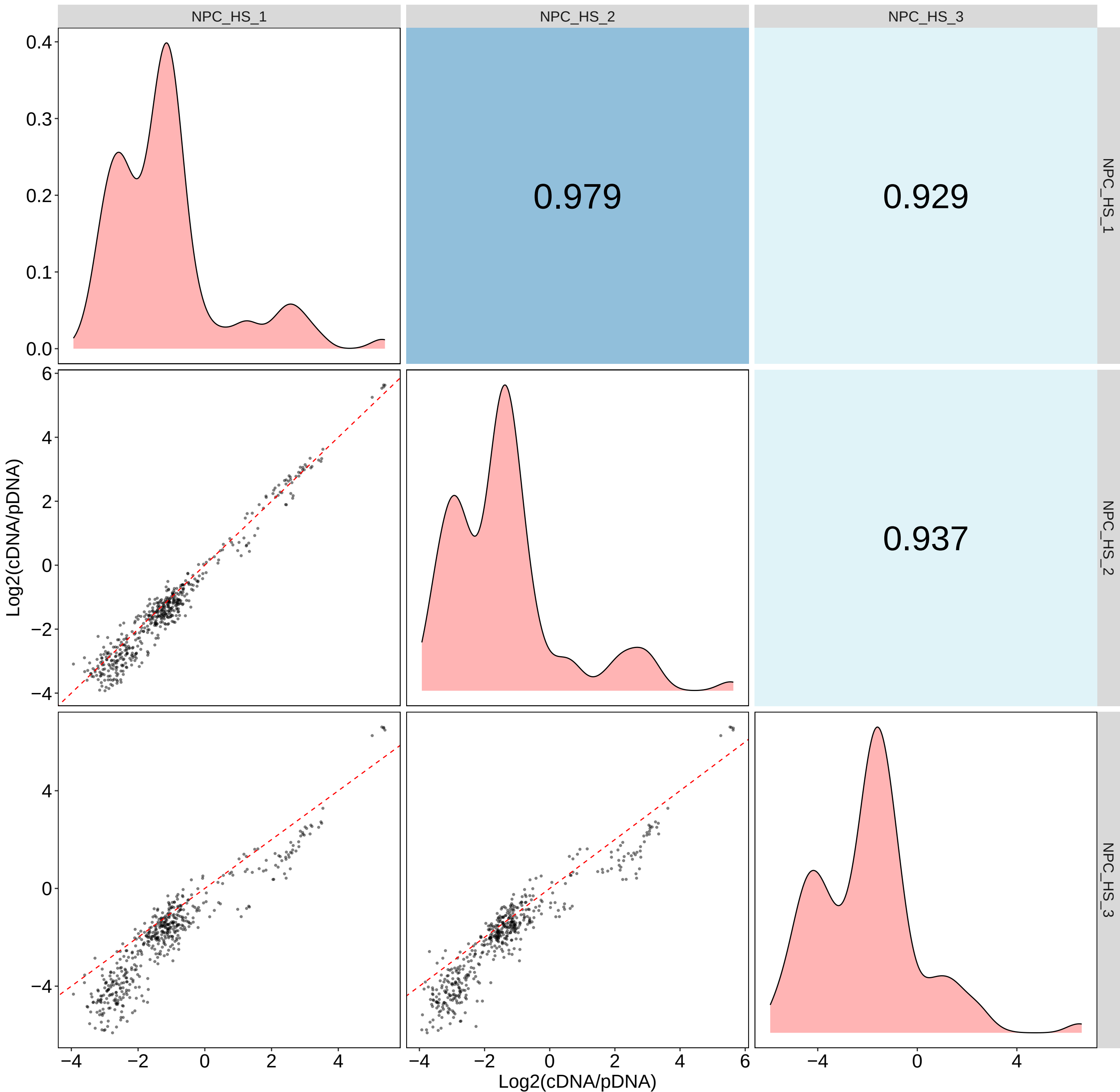
Replicate correlation of NPC_HS
