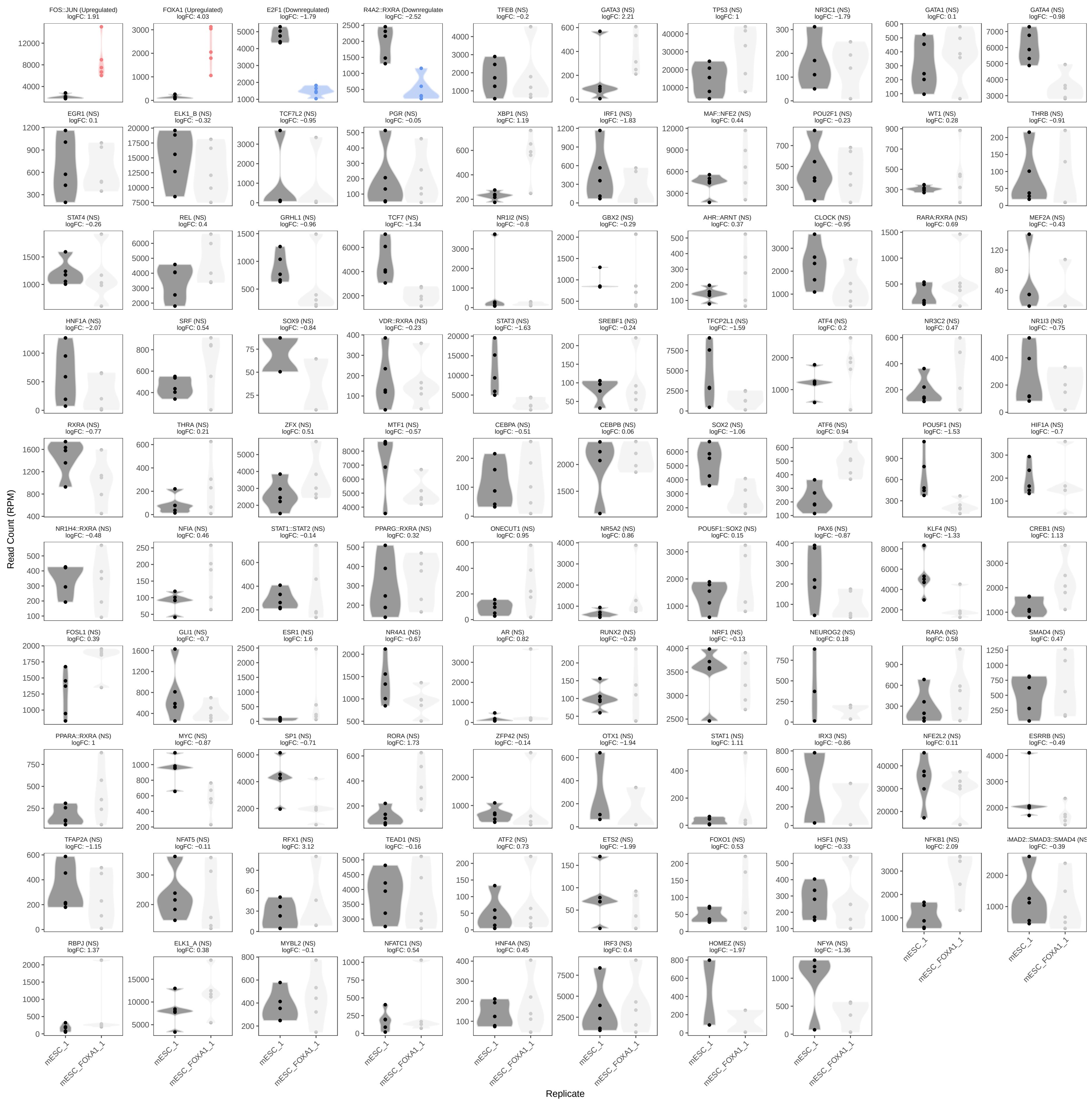
Barcode counts for all TFs (sorted by LogFC*p_adj)
