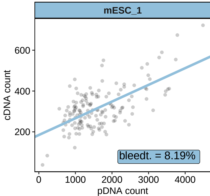
Bleedthrough estimation (Percentage of cDNA counts coming from pDNA)
