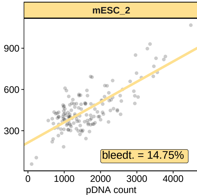
Bleedthrough estimation (Percentage of cDNA counts coming from pDNA)
