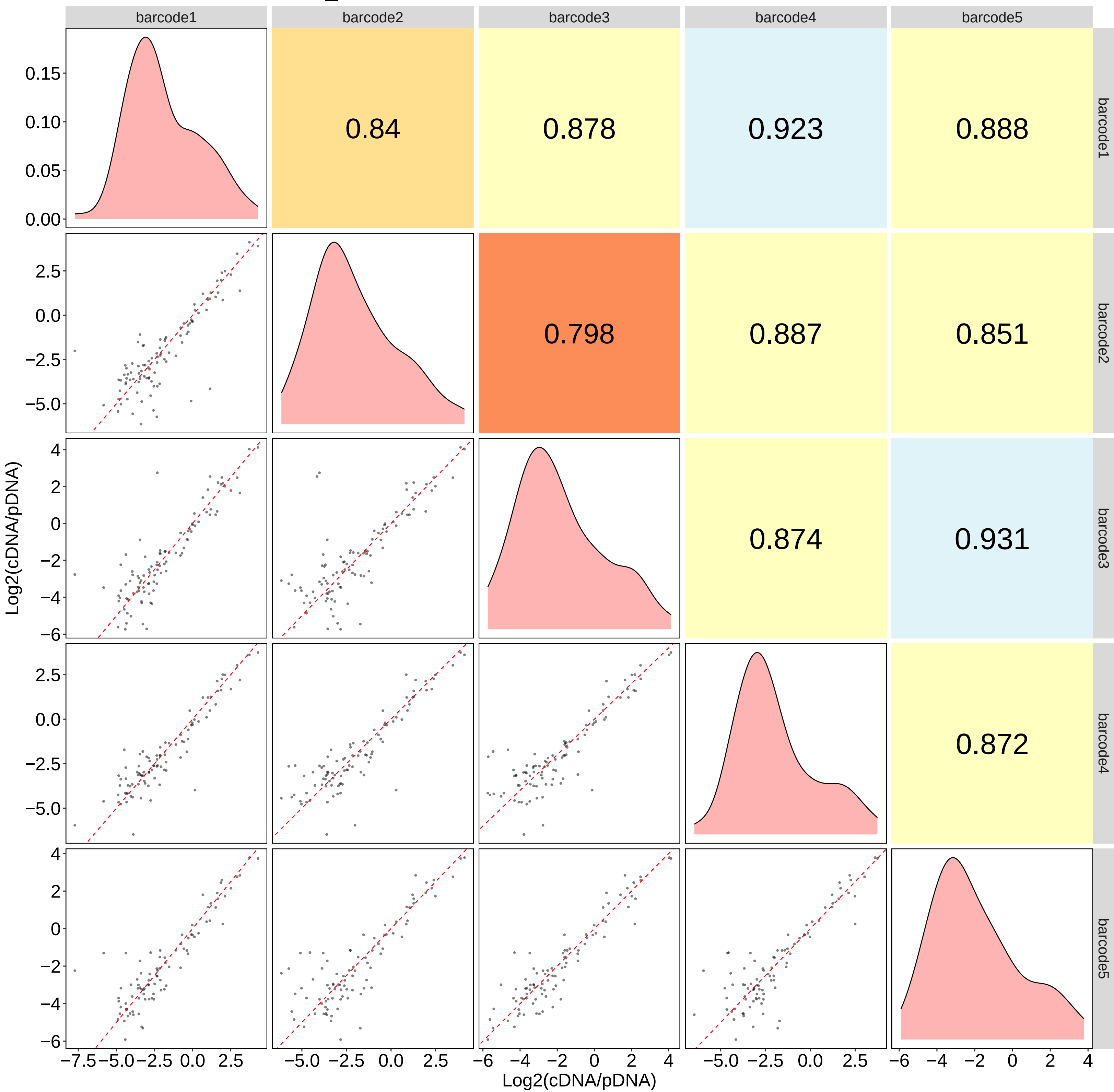
Barcode correlation mESC_3
