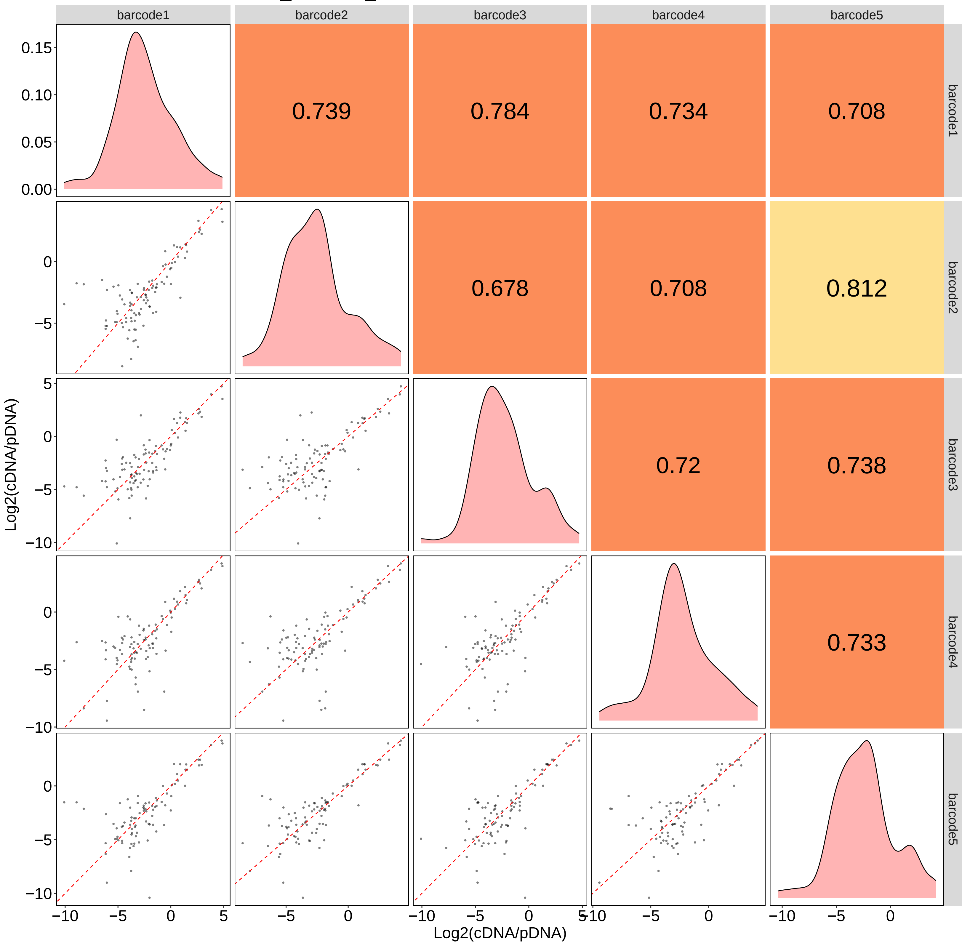
Barcode correlation mESC_POU5F1_2
