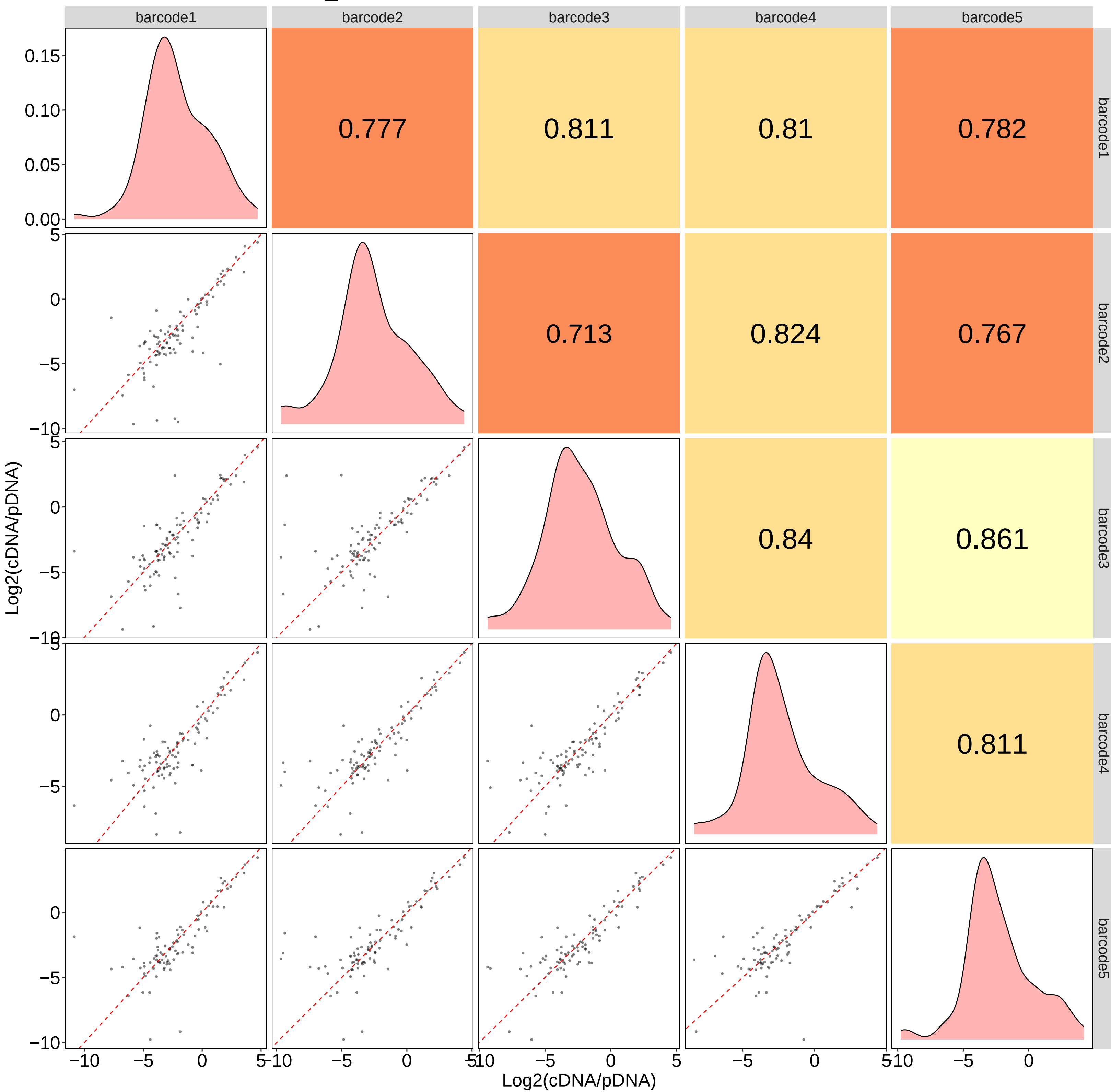
Barcode correlation mESC_2
