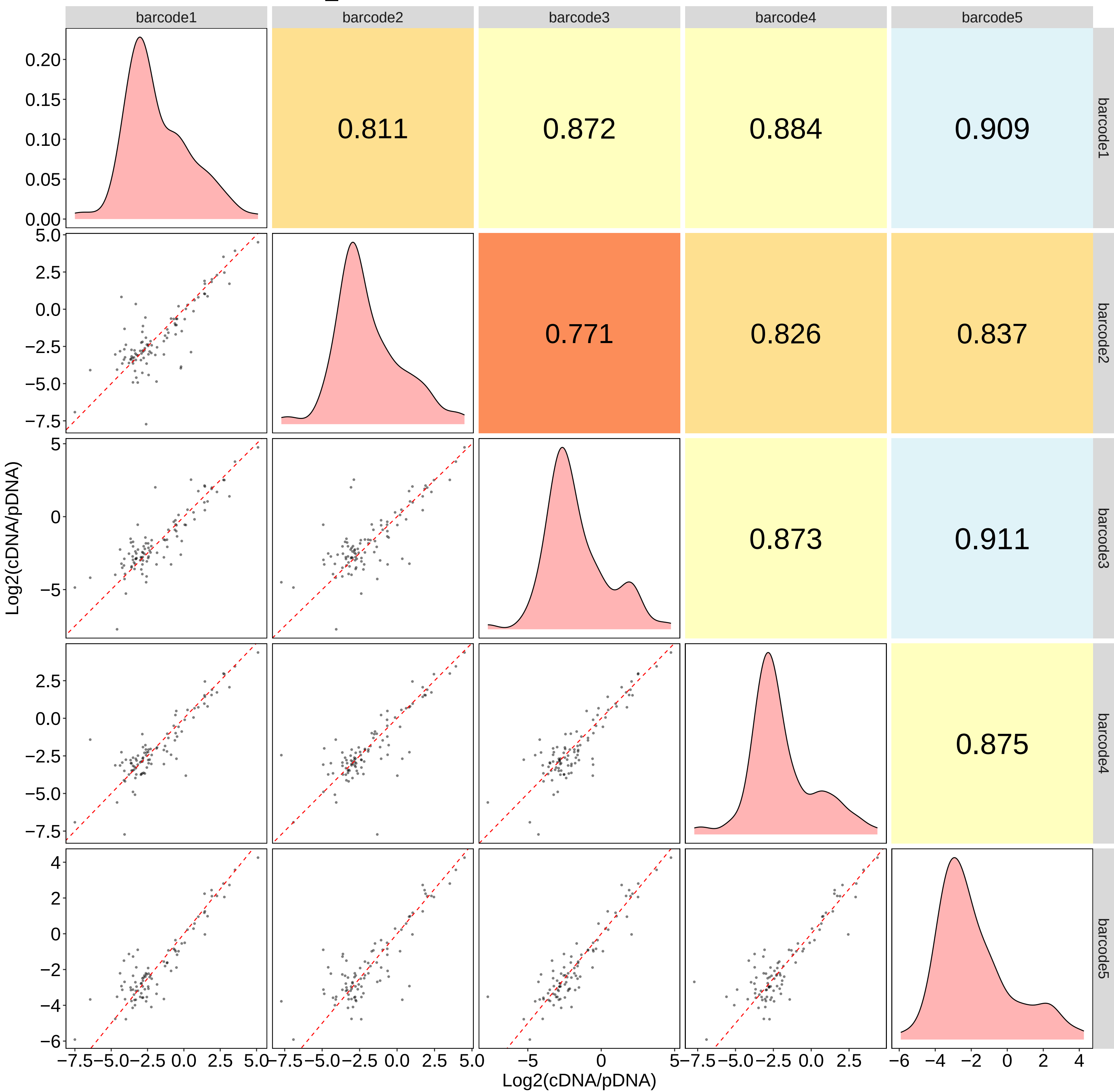
Barcode correlation mESC_1
