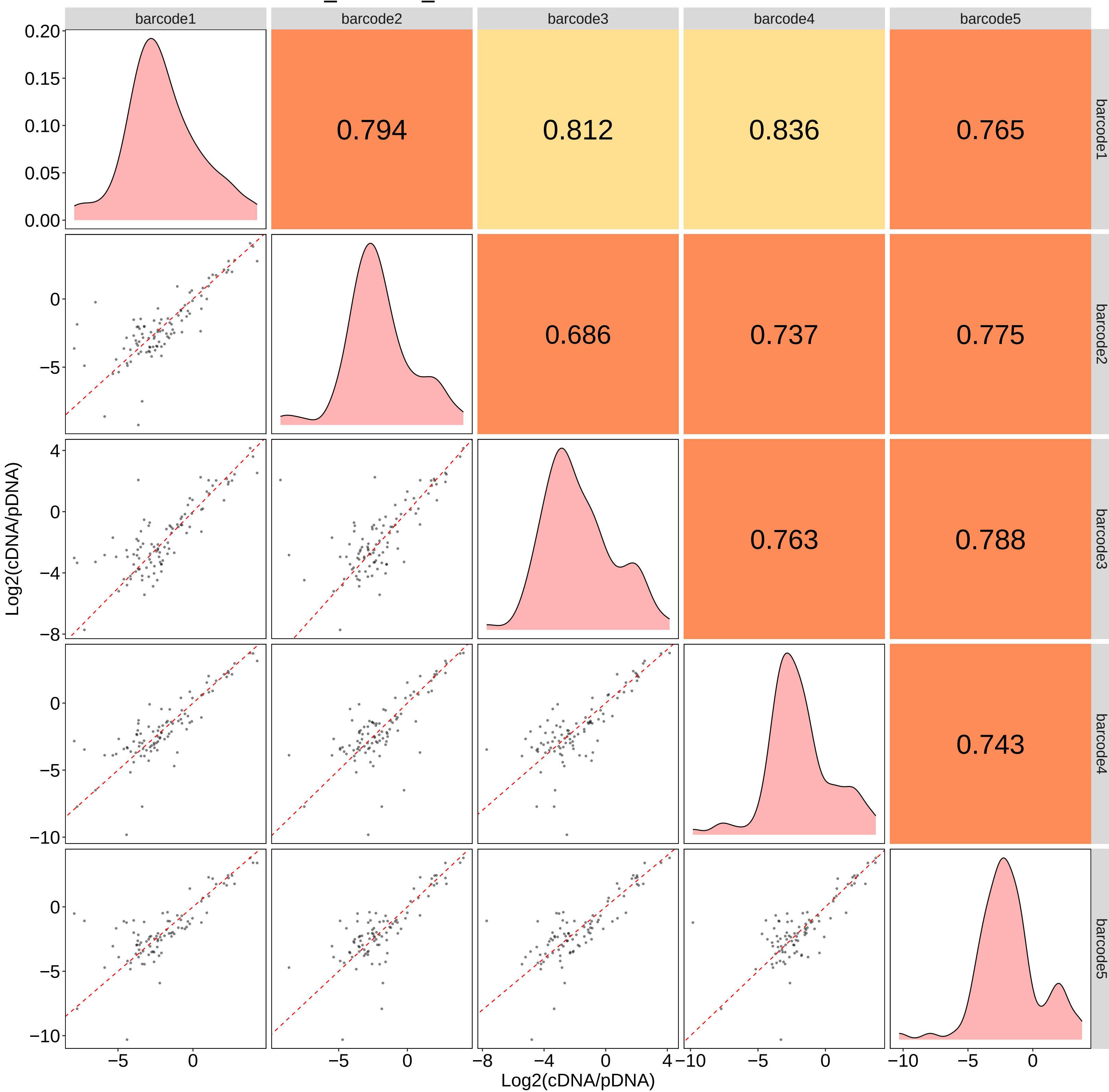
Barcode correlation mESC_POU5F1_3
