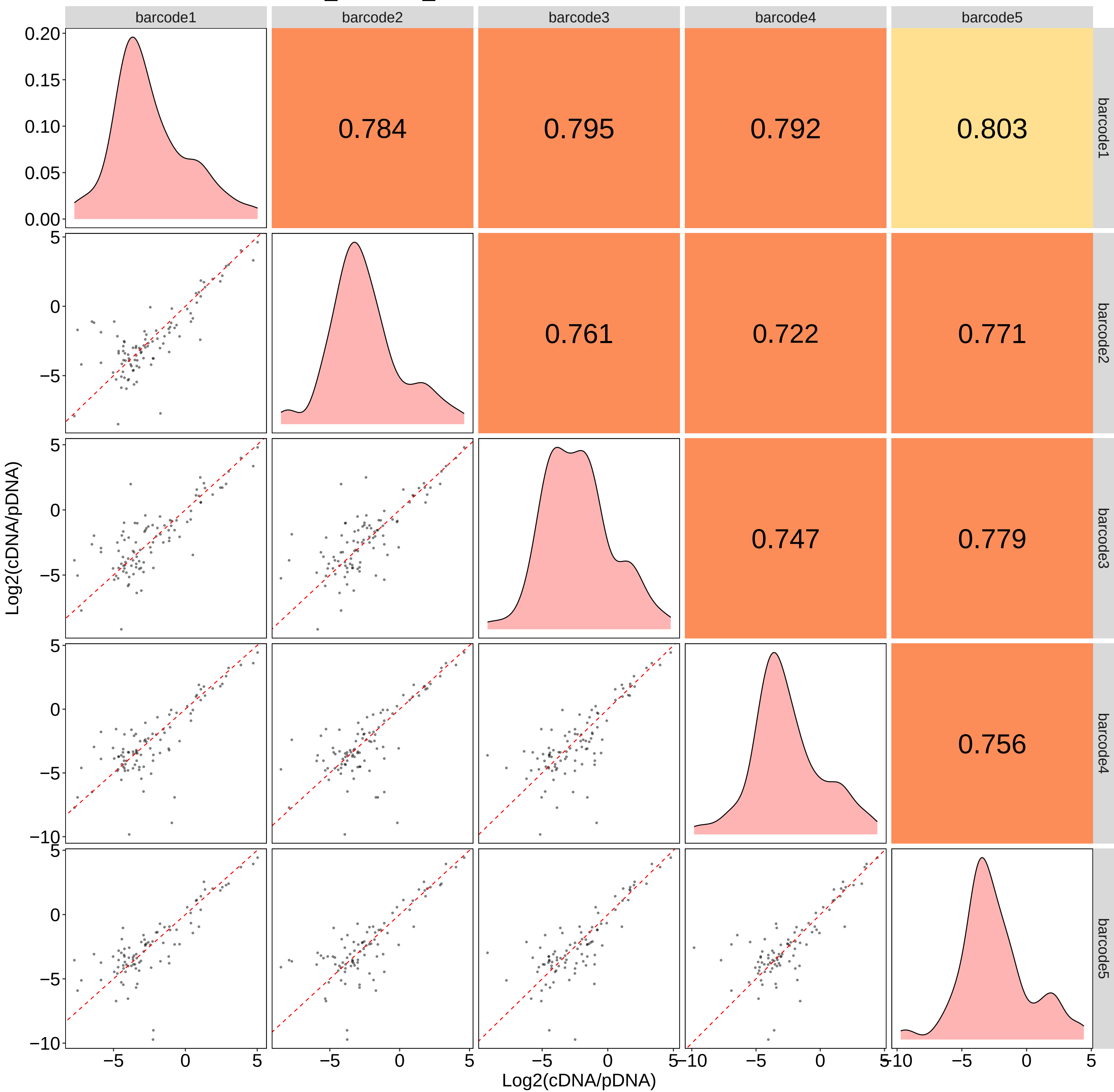
Barcode correlation mESC_POU5F1_1
