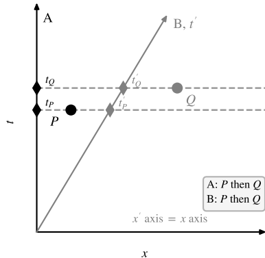
(a) Newtonian: one global time
