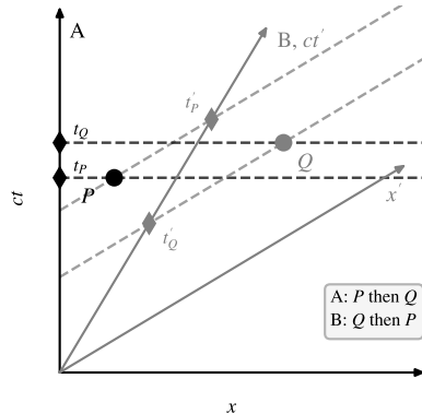
(b) Special relativity: x' tilts with ct'
