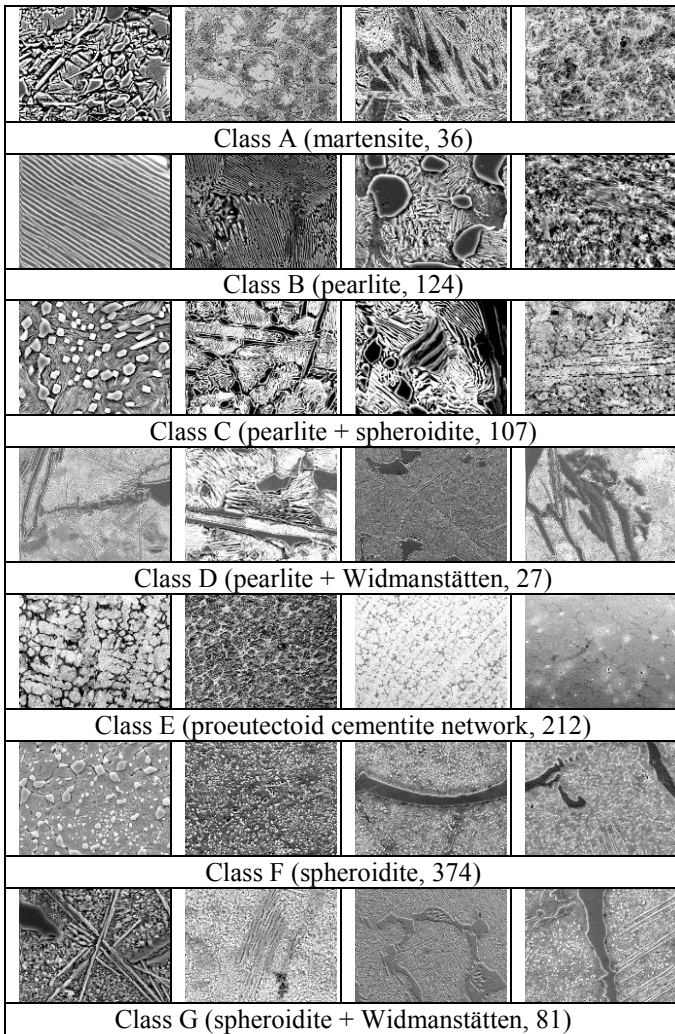
Fig. 1. Typical images of microstructures in UHCS associated with Classes A-G.
