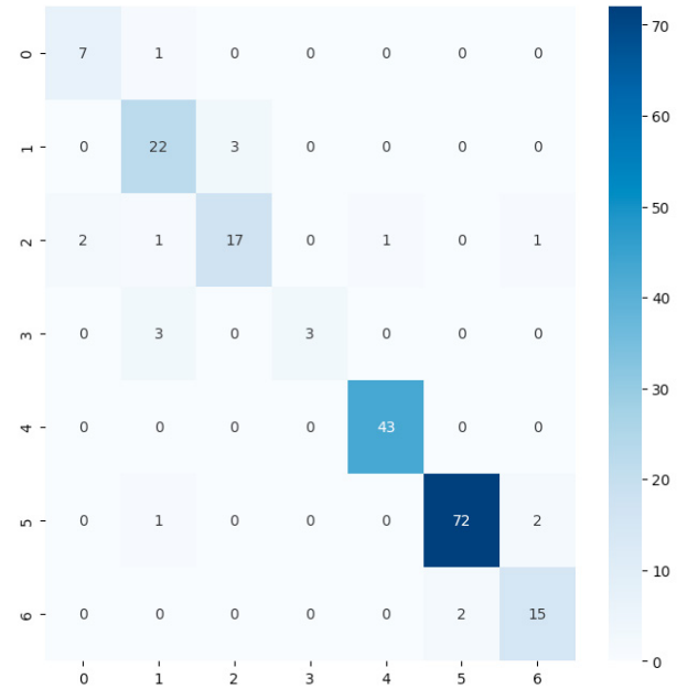
Fig. 4. Confusion matrix on test set for ViT_L32.
