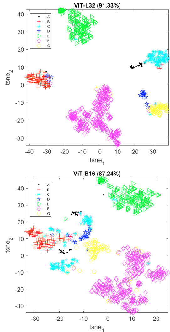
Fig. 2. t -SNE score plot of the features extracted from the ViT models.
