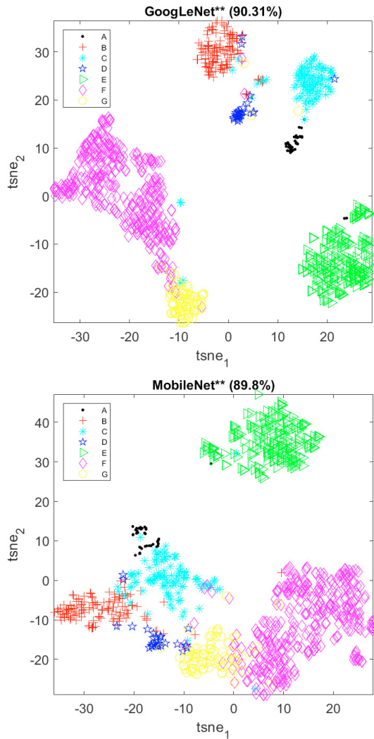
Fig. 3. t-SNE score plot of the features extracted from the CNN models.
