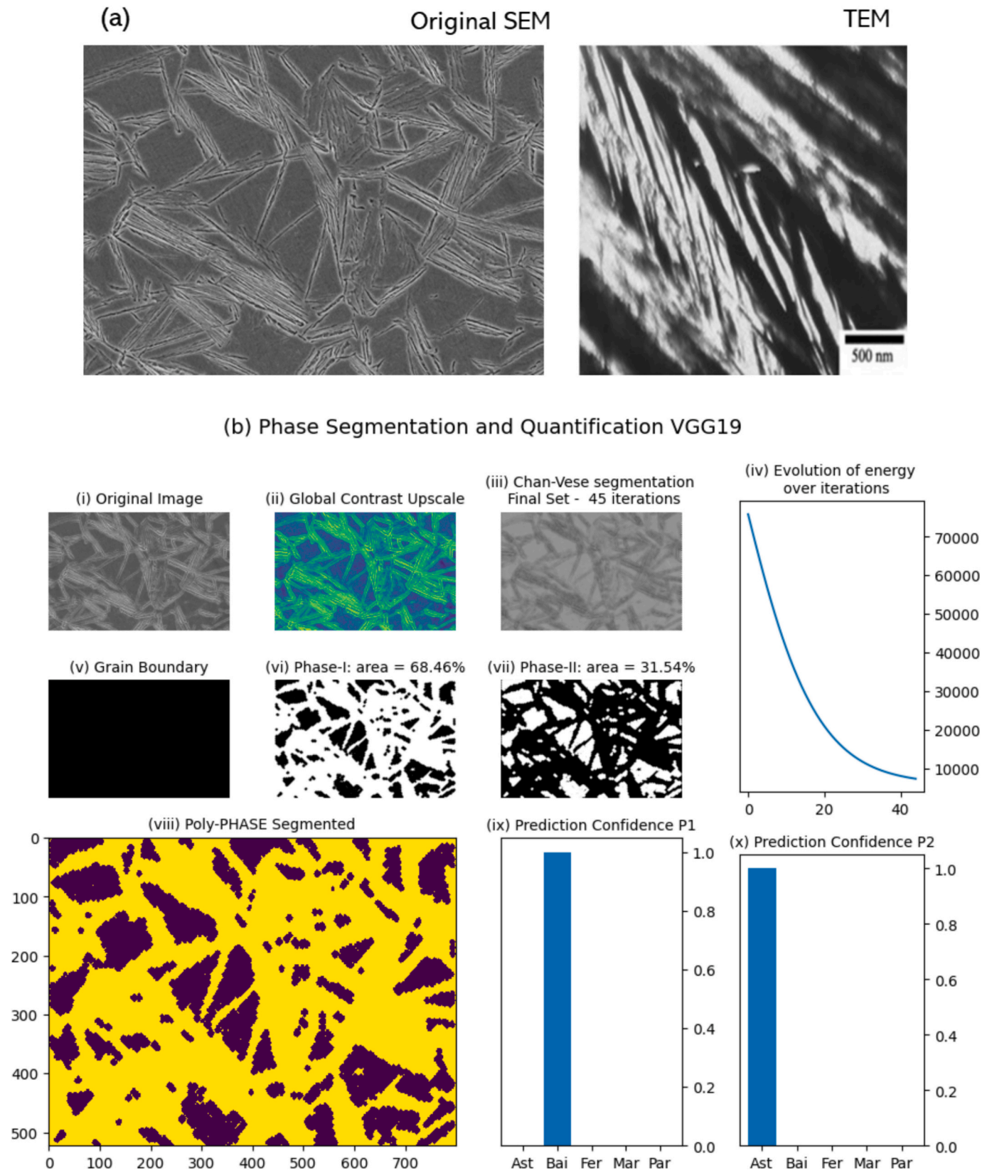
Fig. 10. Demonstration of prediction analysis of a typical case example with a predominantly bainitic-austenite type microstructure. The analysis report produce (a) SEM and TEM micrograph of the original bainite-austenite microstructure representing the ground truth, and (b) referring the sequence of segmented images: (i) original micrograph, (ii) global contrast upscaled, (iii) Chan-Vese (CV) final segmentation result, (iv) evolution of CV energy over 50 iterations, (v) grain boundary (vi and vii) phase masked. (viii) Final segmented microstructure, (ix and x) prediction probability of the identified phase.
