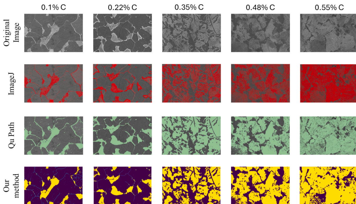
Fig. 18. Segmentation results are obtained from two popular open-source software, namely ImageJ and QuPath, and compared with the proposed model. From left to right, the carbon percentage increases from 0.1 % C to 0.55 % C.
