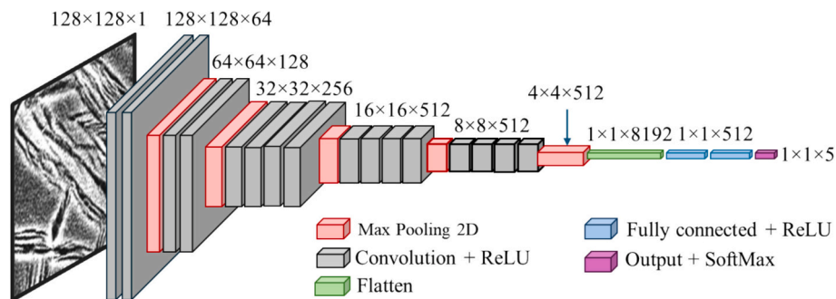
Fig. 3. The schematic of the VGG-19 model is used for the classification of patches belonging to five distinct phases, namely ferrite, pearlite, austenite, bainite, and martensite.
