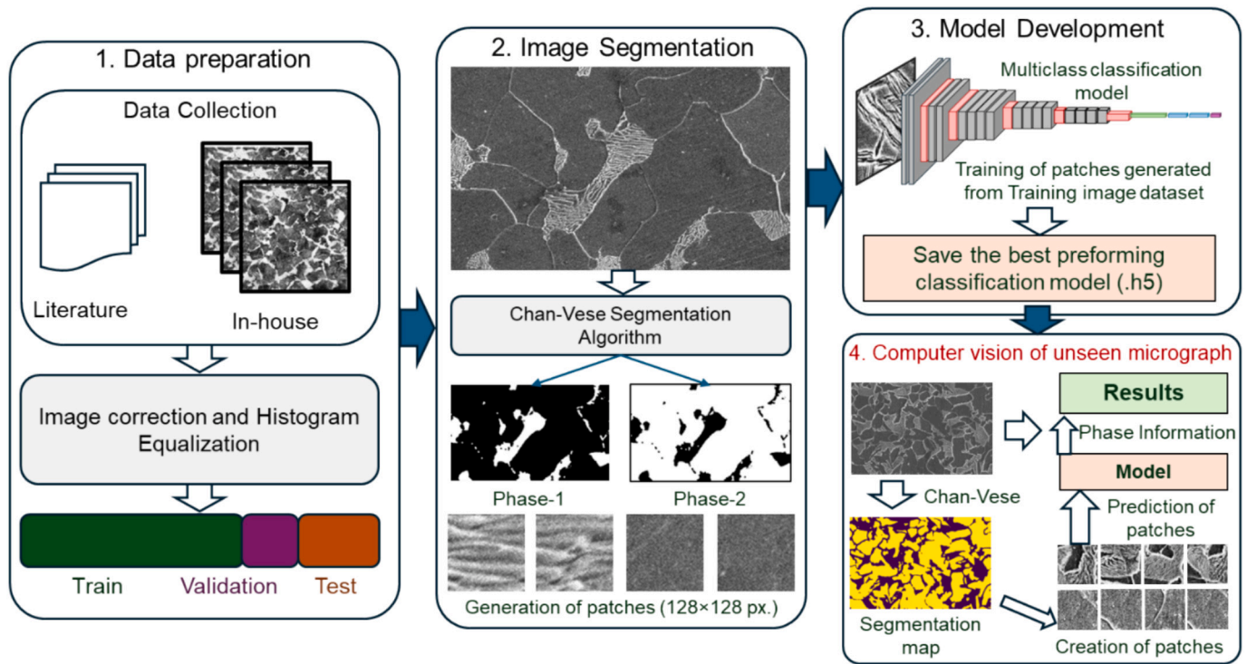
Fig. 1. Schematic representation of image segmentation and classification model framework proposed for digital recognition of phase constituents such as ferrite, pearlite, austenite, bainite, and martensite in SEM micrograph image of steel. The first block demonstrates the data collection splitting while the second block explains the segmentation of microstructure and generation of patches of segmented phases. The latter block represents the DL model training with phase patches and prediction of phase constitution in an unseen microstructure.
