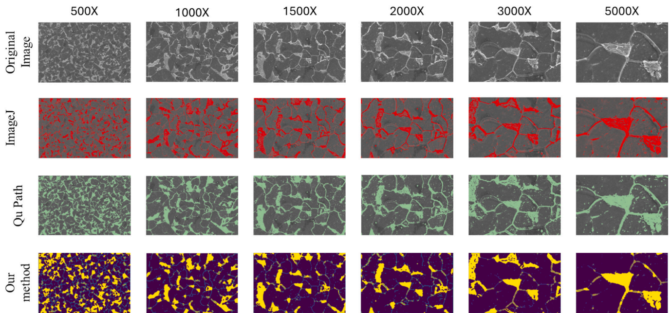
Fig. 16. Segmentation results are obtained from two popular open-source software namely ImageJ and QuPath and compared with the proposed model. From left to right magnification increases from 500\times to 5000\times .
