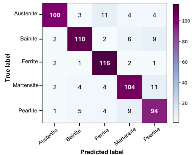
Fig. 8. The confusion matrix shows the overall performance based on the VGG-19 model on the testing data.
