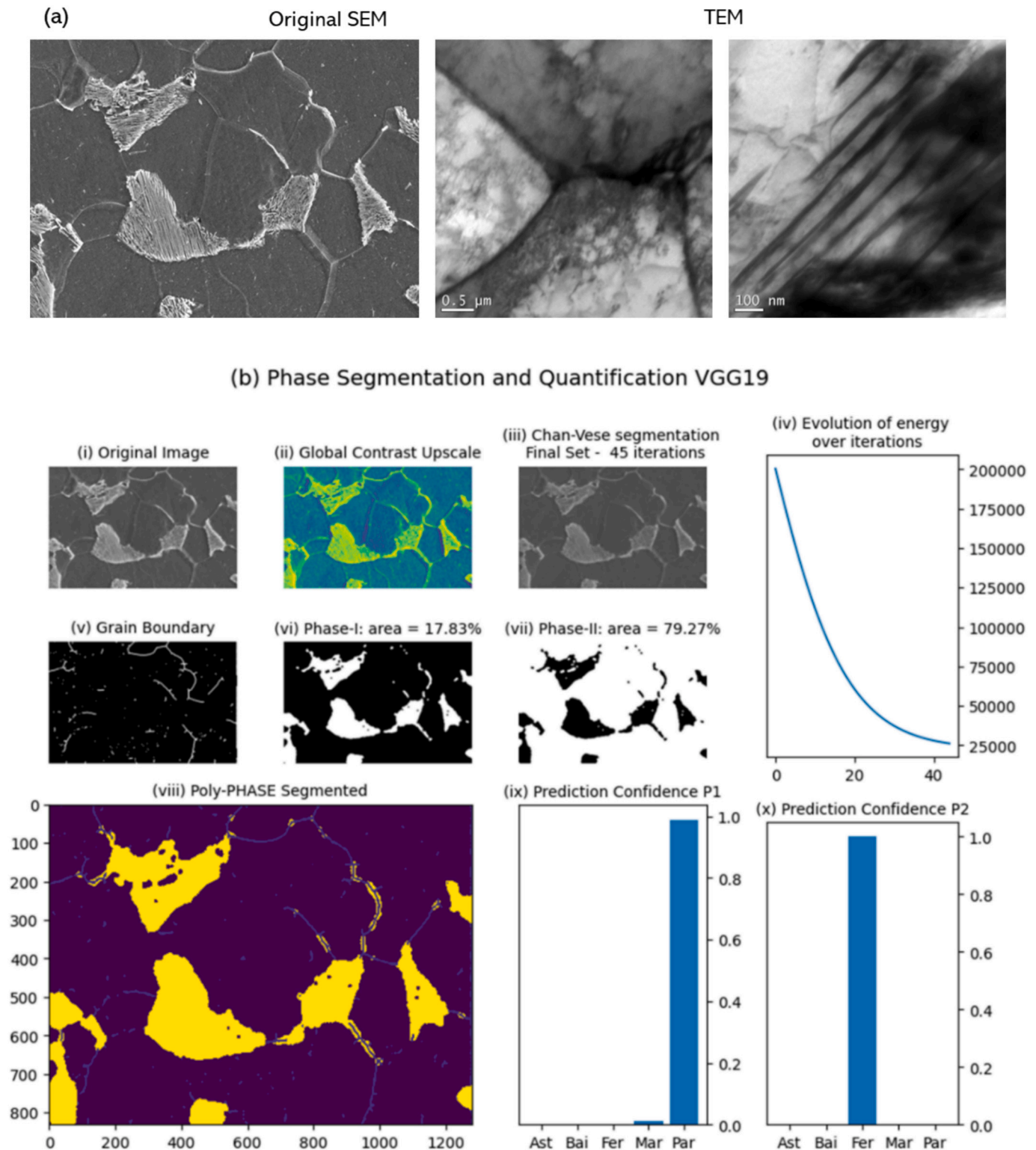
Fig. 11. Demonstration of prediction analysis of a typical case example with a predominantly ferrite-pearlite type microstructure. The analysis report produce (a) SEM and TEM micrograph of the original ferrite-pearlite microstructure representing the ground truth, and (b) referring the sequence of segmented images: (i) original micrograph, (ii) global contrast upscaled, (iii) Chan-Vese (CV) final segmentation result, (iv) evolution of CV energy over 50 iterations, (v) grain boundary (vi and vii) phase masked. (viii) Final segmented microstructure, (ix and x) prediction probability of the identified phase.
