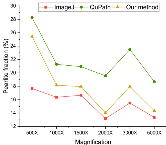
Fig. 17. Comparison of the pearlite phase fraction obtained from ImageJ, QuPath, and the proposed model with the increase of magnification.
