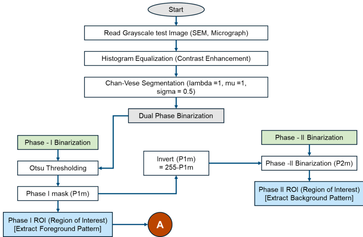
Fig. 2. The schematic procedure to segment the microstructure using Chan-Vese segmentation technique after that extraction of region of interest.
