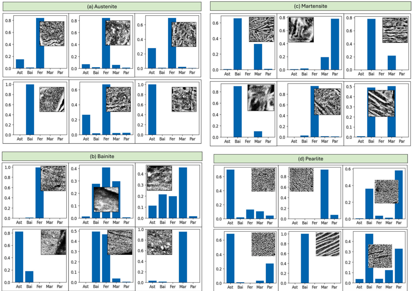
Fig. 9. The predicted probability density was obtained from the last layer of VGG-19 classification. In this fig. Major wrong prediction of the patches is depicted. (a) probability plot for wrong prediction of the austenite patches, (b) probability plot for wrong prediction of the bainite patches, (c) probability plot for wrong prediction of the martensite patches, and (d) probability plot for wrong prediction of the pearlite patches.
