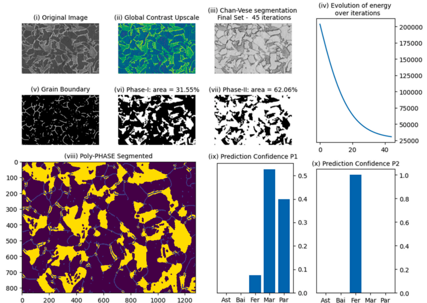
Fig. 15. A typical example of the heavily confused prediction made by the model, the micrograph belongs to a pearlite-ferrite based system but is predicted as a martensite-ferrite based system.
