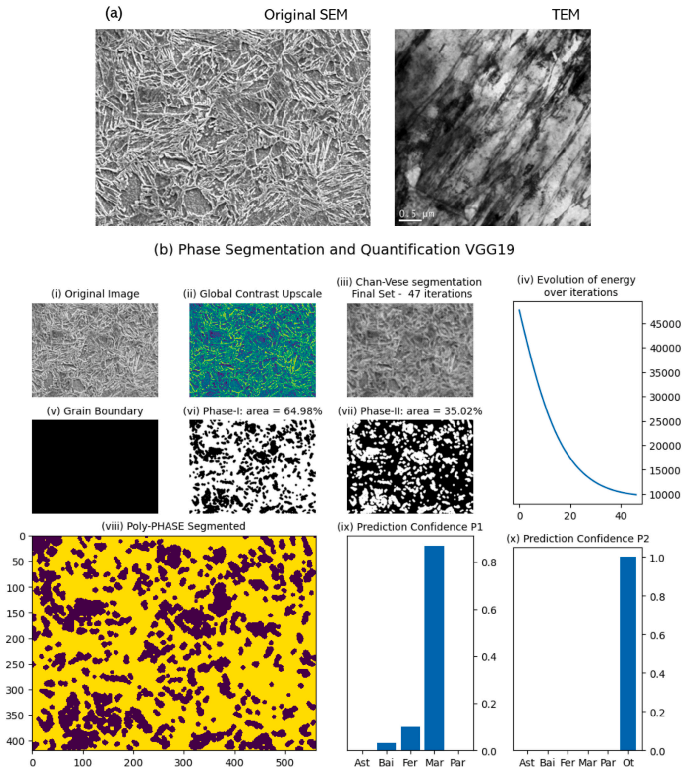
Fig. 12. Demonstration of prediction analysis of a typical case with a predominantly martensite-bainite type microstructure. The analysis report produce (a) SEM and TEM micrograph of the original martensite-bainite microstructure representing the ground truth, and (b) referring the sequence of segmented images: (i) original micrograph, (ii) global contrast upscaled, (iii) Chan-Vese (CV) final segmentation result, (iv) evolution of CV energy over 50 iterations, (v) grain boundary (vi and vii) phase masked. (viii) Final segmented microstructure, (ix and x) prediction probability of the identified phase.
