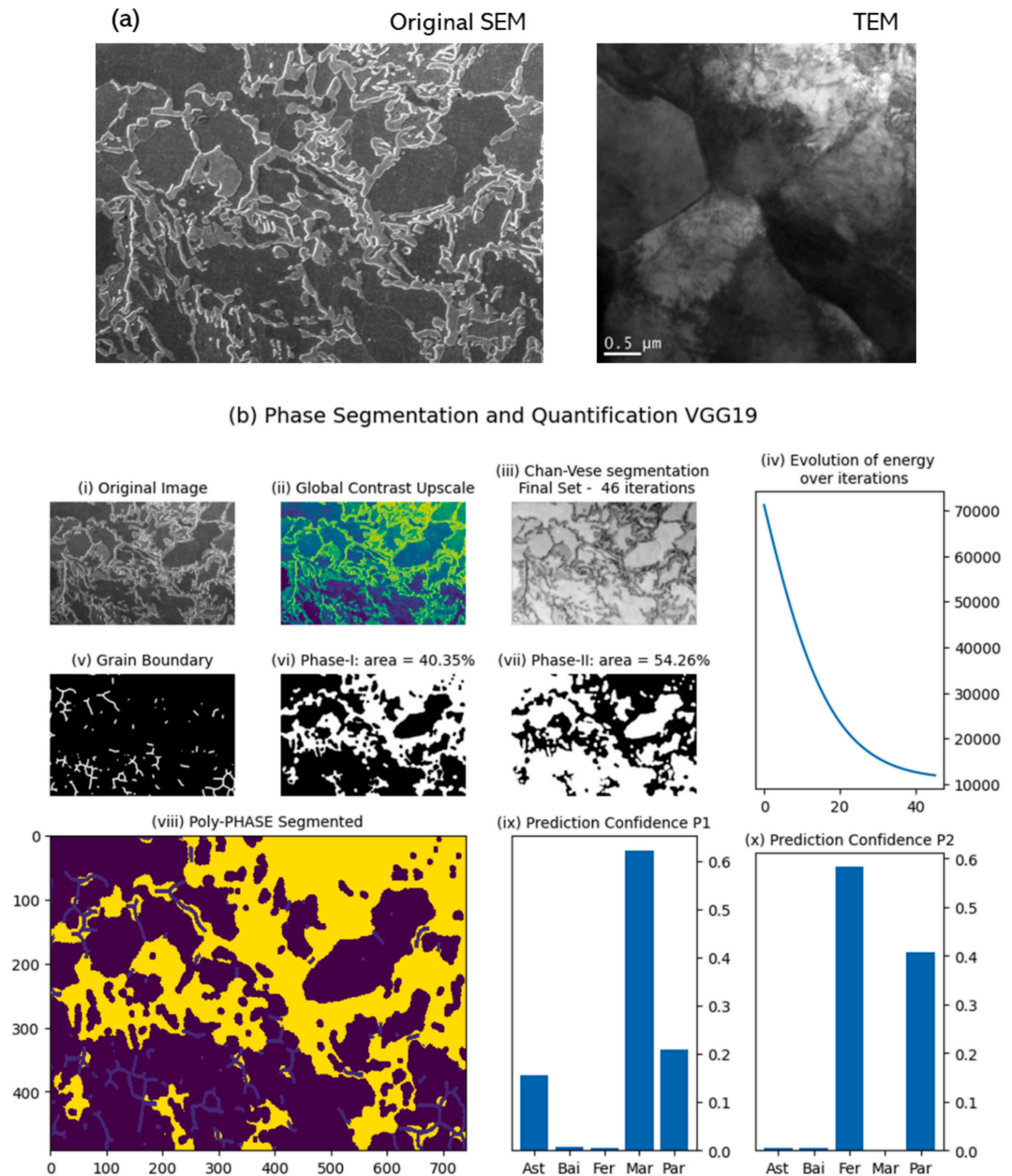
Fig. 13. Demonstration of prediction analysis of a typical case example with a predominantly ferrite-martensite type microstructure. The analysis report produce (a) SEM and TEM micrograph of the original ferrite-martensite microstructure representing the ground truth, and (b) referring the sequence of segmented images: (i) original micrograph, (ii) global contrast upscaled, (iii) Chan-Vese (CV) final segmentation result, (iv) evolution of CV energy over 50 iterations, (v) grain boundary (vi and vii) phase masked. (viii) Final segmented microstructure, (ix and x) prediction probability of the identified phase.
