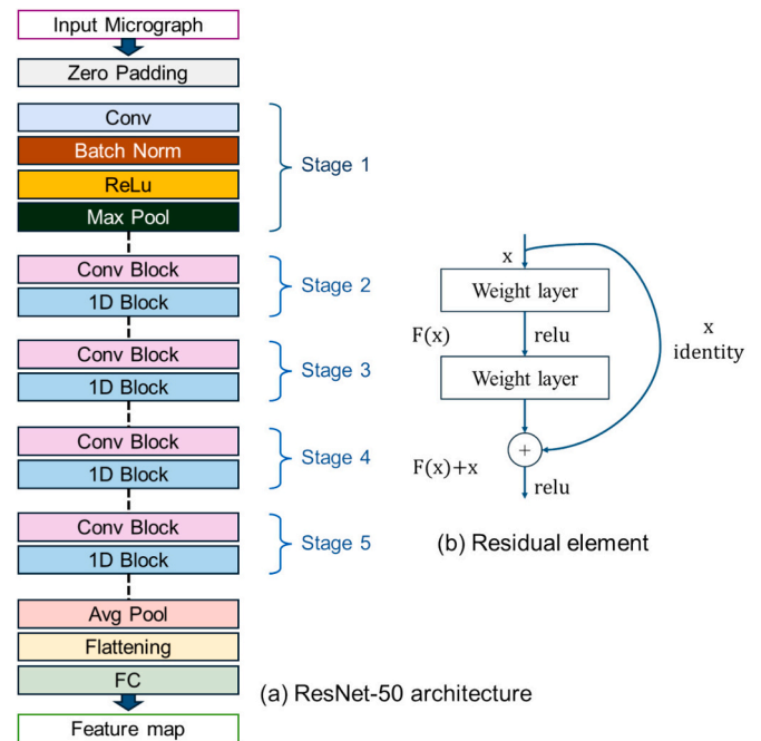
Fig. 4. (a) Architecture of ResNet50 containing an initial convolutional layer, five stage of residual blocks, and final layers for classification of phases. A Residual block starts with 1 \times 1 convolution layer, followed by a 3 \times 3 convolution layer and with 1 \times 1 convolutional layer. The final output is then added to the input via a residual connection as shown in (b).
