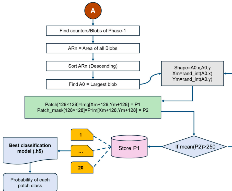
Fig. 6. The step-by-step procedure for extraction and classification of the patches. First the microstructure was segmented into distinct phases as depicted in Fig. 2. The contours/blobs were sorted in descending order of blobs' area. After that largest blob was used to extract the patches followed by the classification task was performed to classify the patches.
