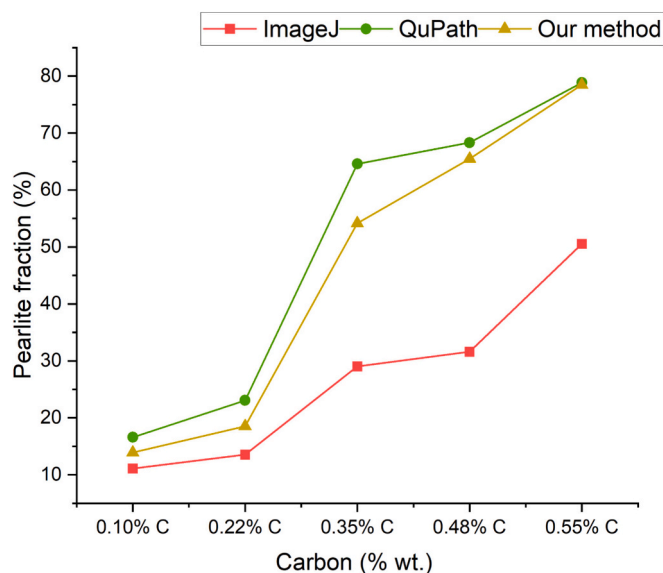
Fig. 19. Comparison of the pearlite phase fraction obtained from ImageJ, QuPath, and the proposed model with the increase of C (wt%).
