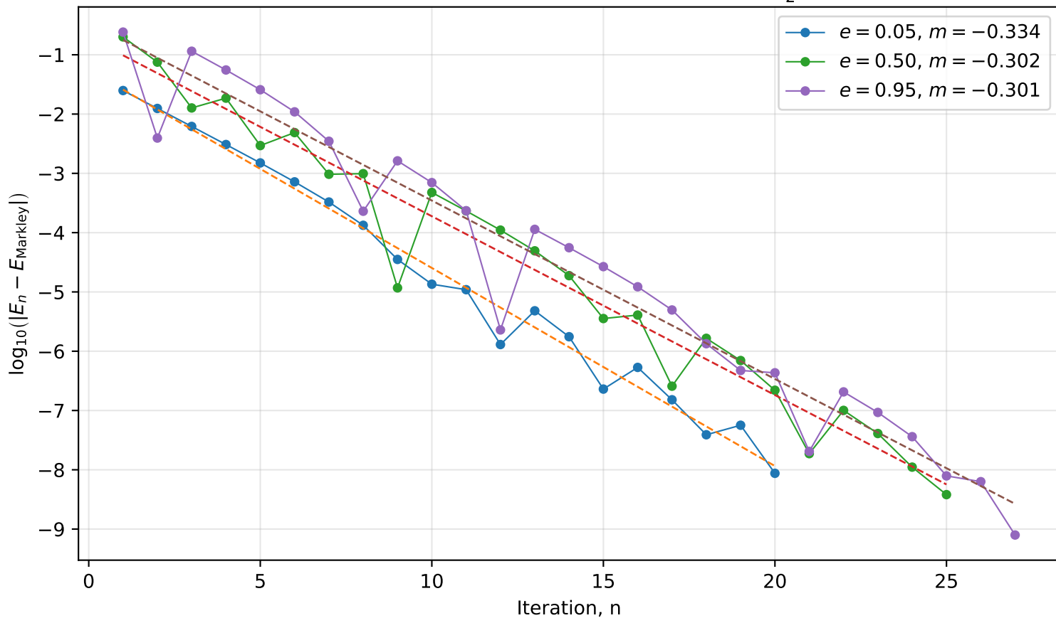
Bisection Convergence History for M = \frac{\pi}{2}
