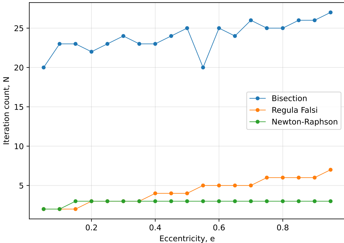
Iteration Count vs Eccentricity for M = \pi/2
