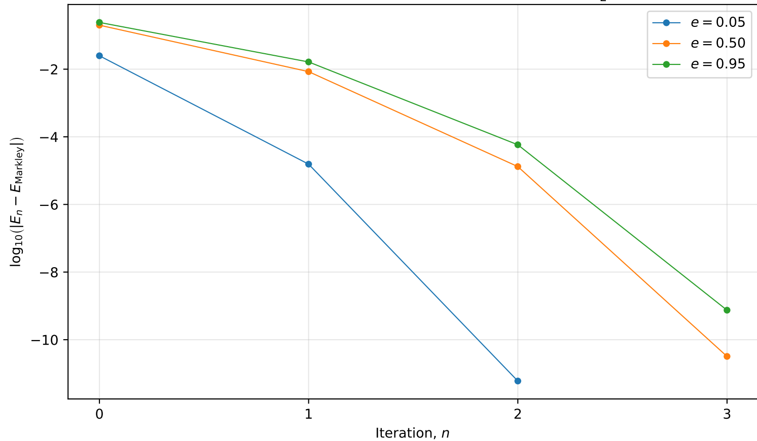
Newton-Raphson Convergence History for M = \frac{\pi}{2}
