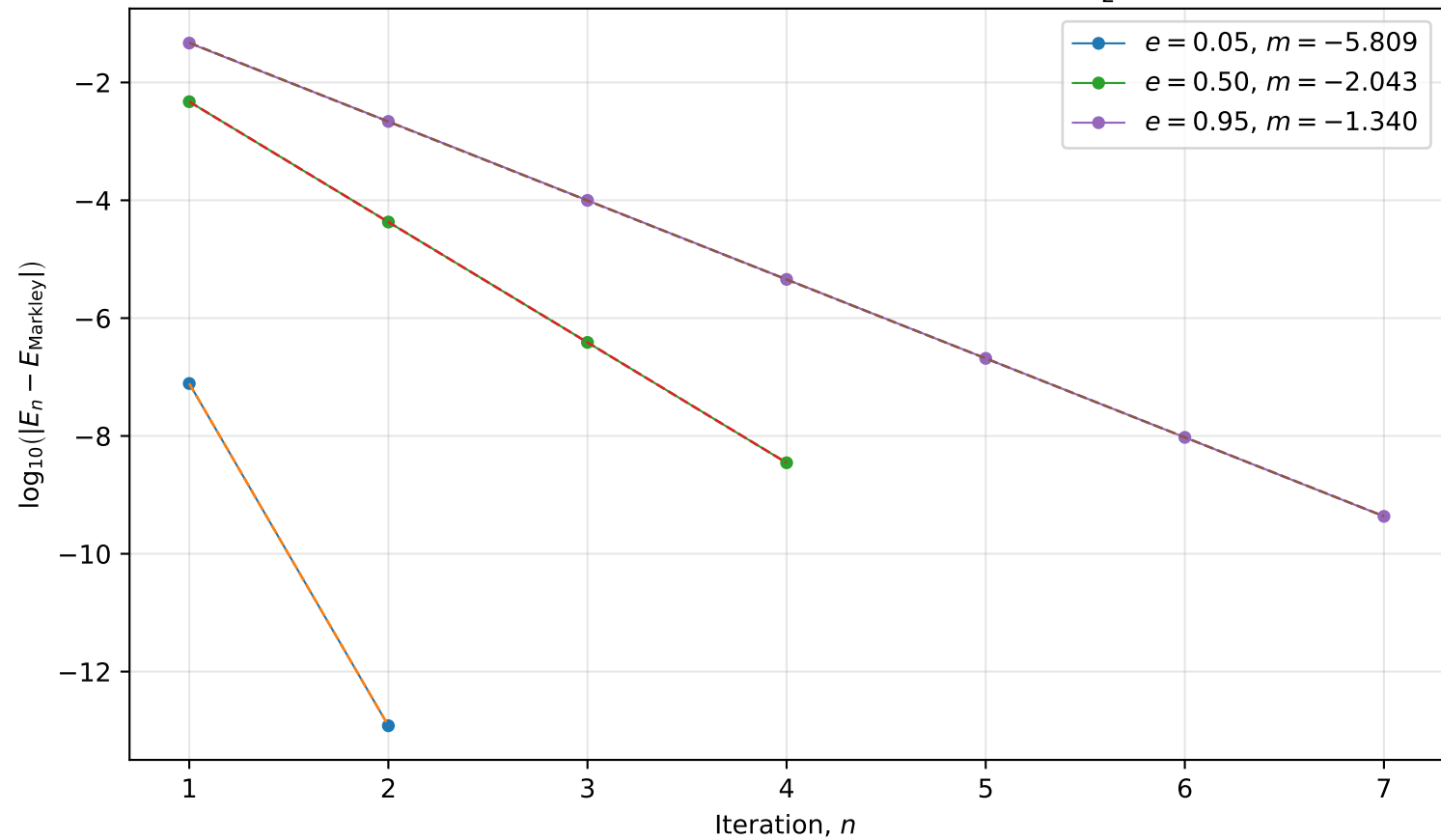
Regula Falsi Convergence History for M = \frac{\pi}{2}
