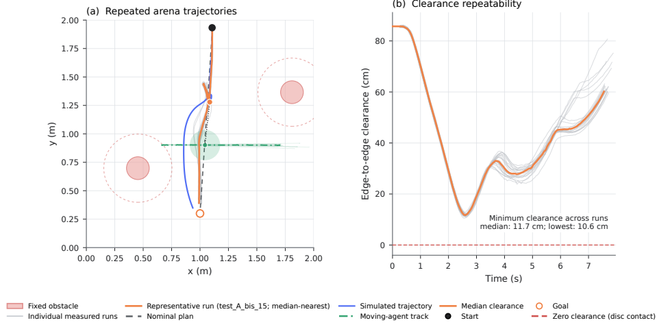
Fig. 6 Twenty physical runs with one moving agent (Online Resource 1): arena paths and conservative edge-to-edge clearance. Zero denotes overlap of the bounding discs, not chassis contact.
