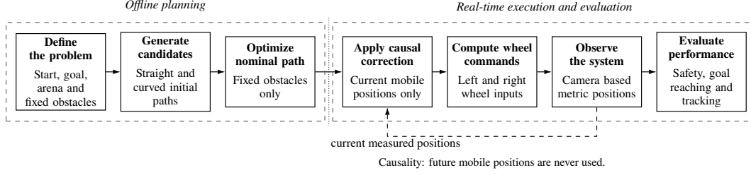
Fig. 2 Global-local architecture and offline/online boundary. Only current and retained past observations of moving agents enter the local corrector.
