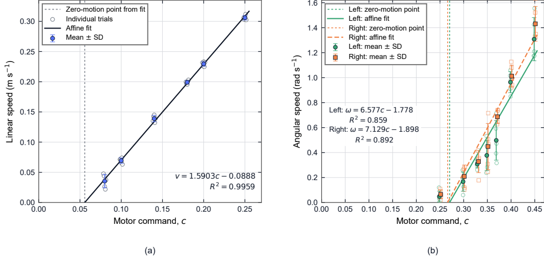
Fig. 4 Open-loop drivetrain characterisation: translation over thirty trials and rotation over seventy trials. Error bars span one standard deviation over five repetitions; zero-motion points are affine-fit extrapolations.
