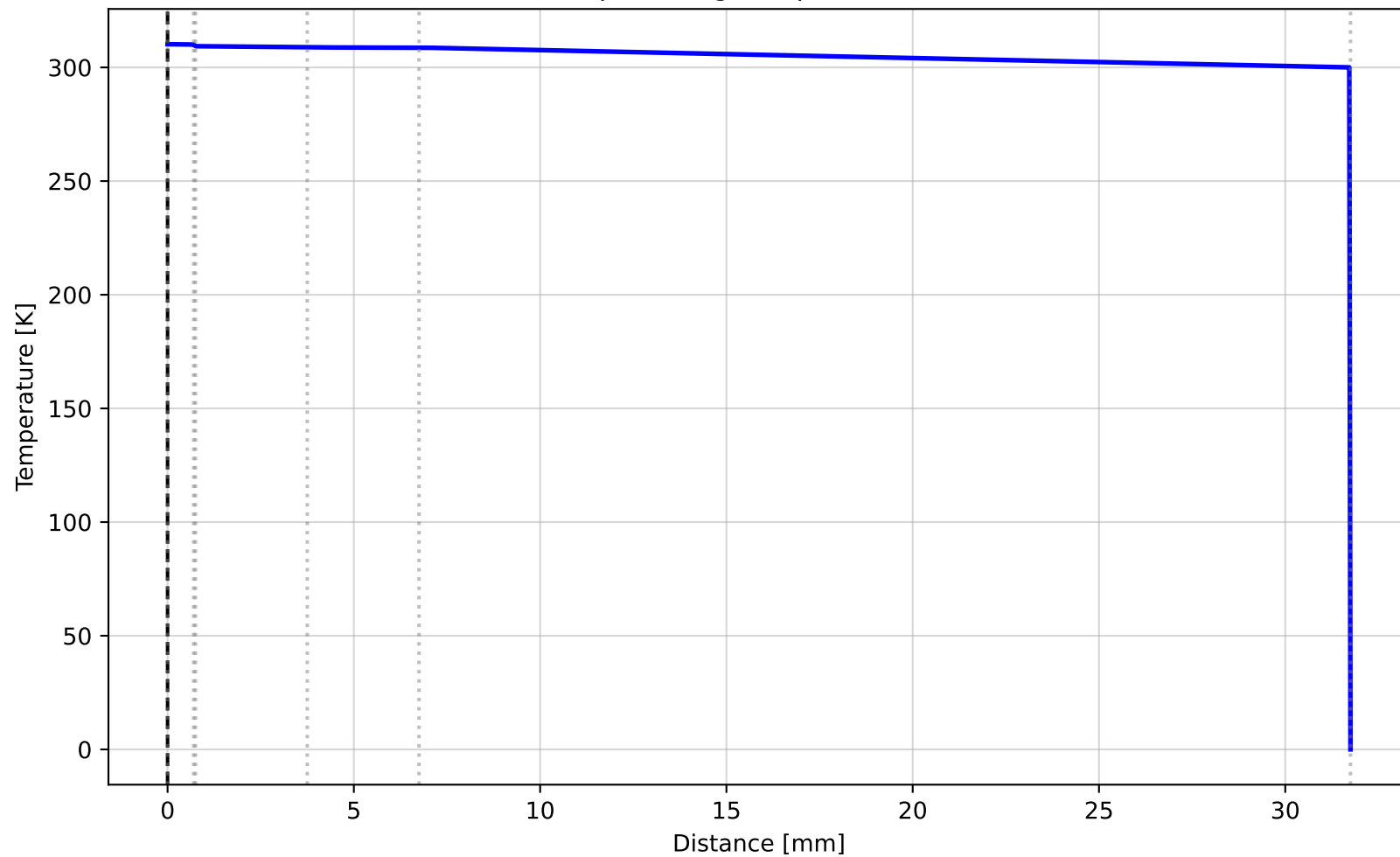
1D Chip Cooling Temperature Profile
