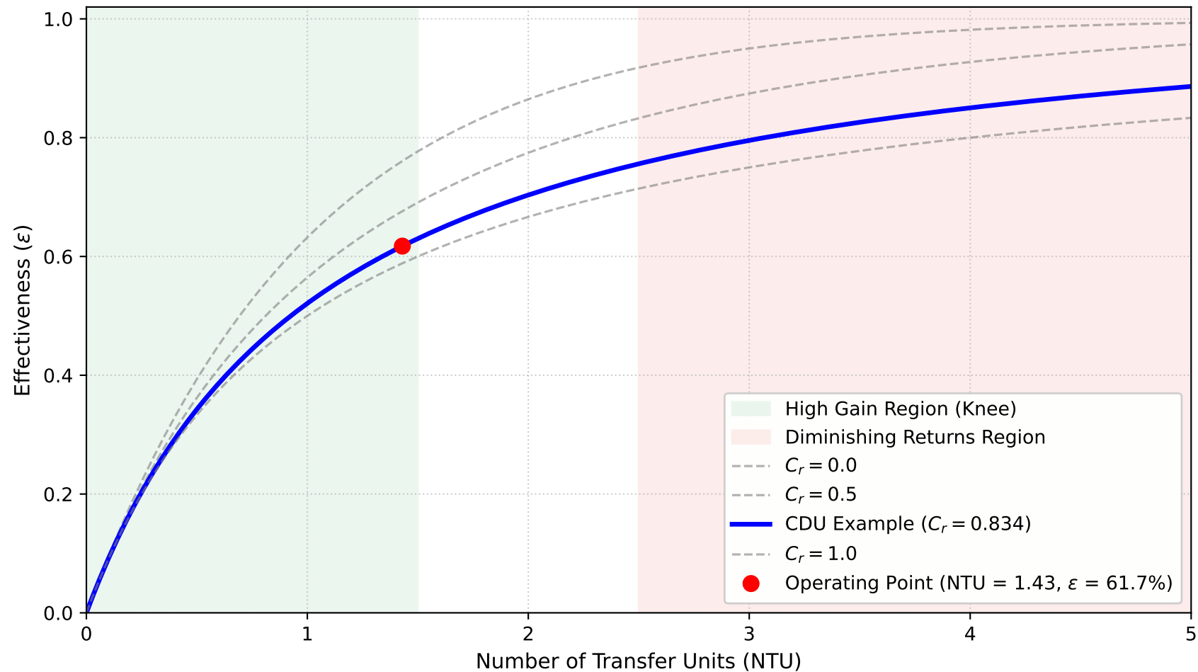
Counter-Flow Effectiveness ( \varepsilon ) vs. NTU
