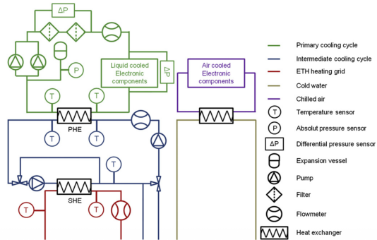
Figure 7: Aquasar: Schematics of the cooling loop [3]. Let us analyze the second law efficiency of the green loop.
