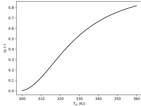
Figure 8: Second-law efficiency of the secondary TCS loop [3].
