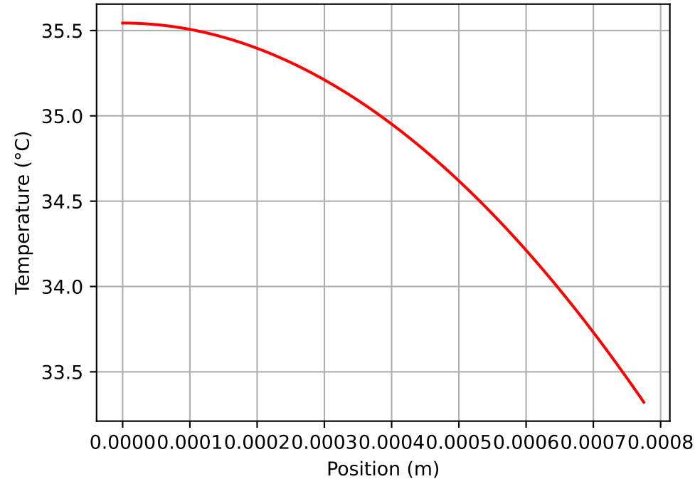
Dye temperature
