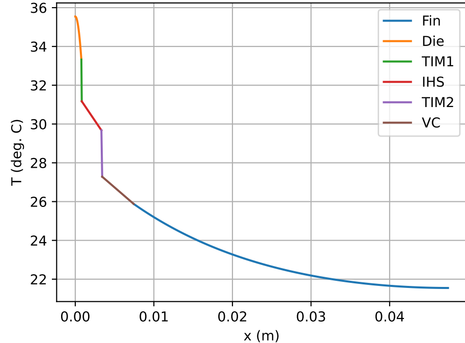
Temperature Distribution in Chip Stack
