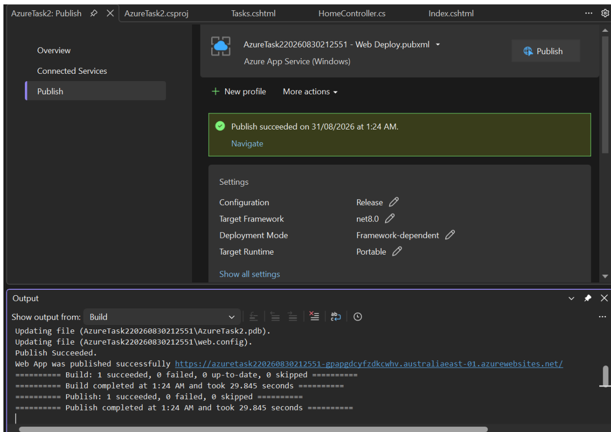
Figure 17: Successful republishing of the application after configuring the health check endpoint.
