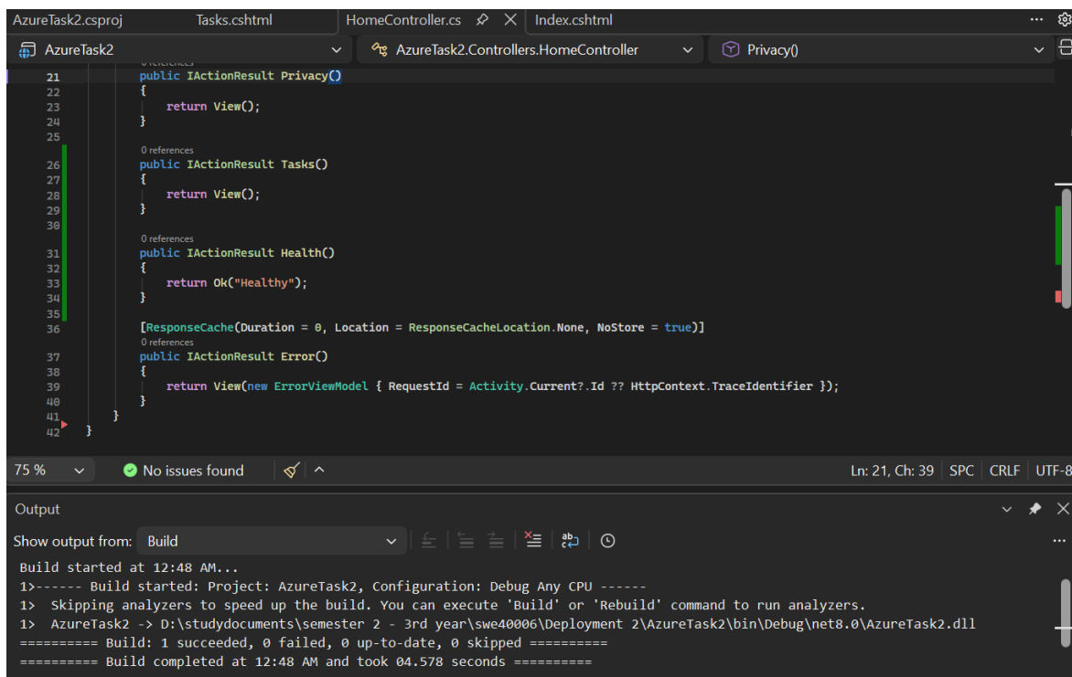
Figure 14: Adding a health check endpoint to the HomeController.
