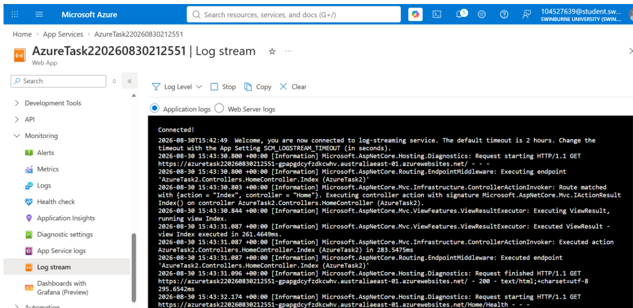
Figure 22: Real-time ASP.NET Core request and diagnostic logs displayed through Azure App Service Log Stream.
