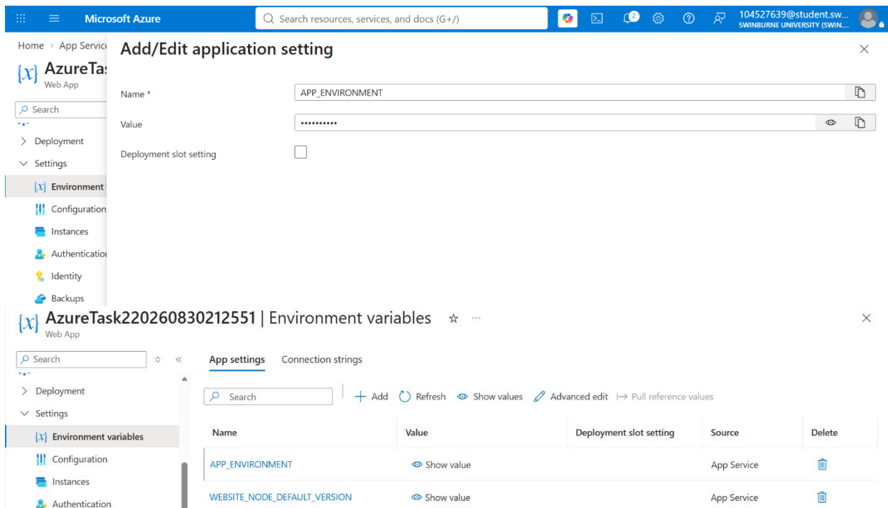
Figure 15: Adding the APP_ENVIRONMENT setting with the value Production in Azure App Service.
