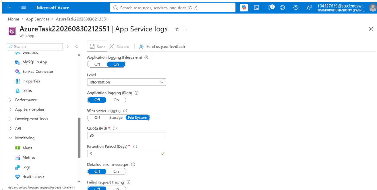
Figure 20: Azure App Service application and web server logging configuration.
