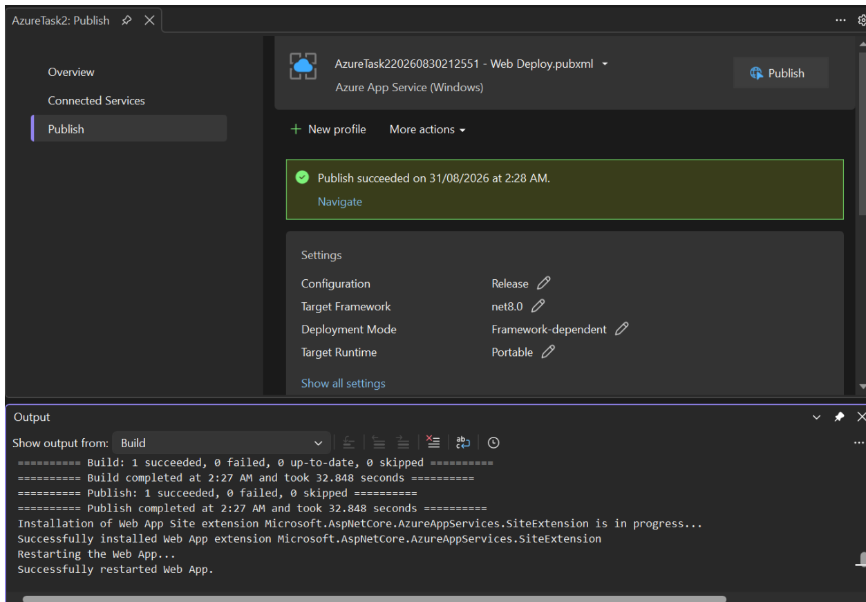
Figure 11: Successfully publication of the .NET 8 ASP.NET Core application to Azure Cloud services.
