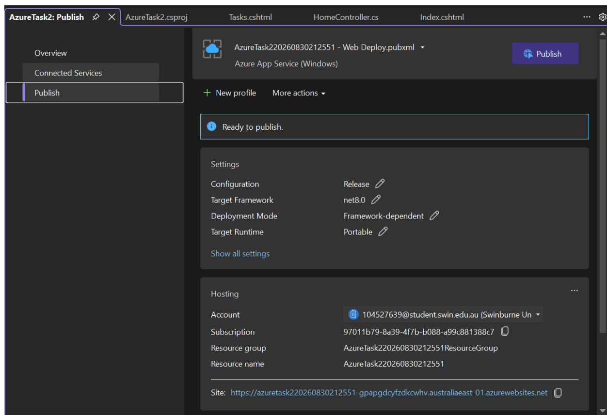
Figure 9: Visual Studio publish configuration for the .NET 8 application targeting Azure App Service in Australia East.
