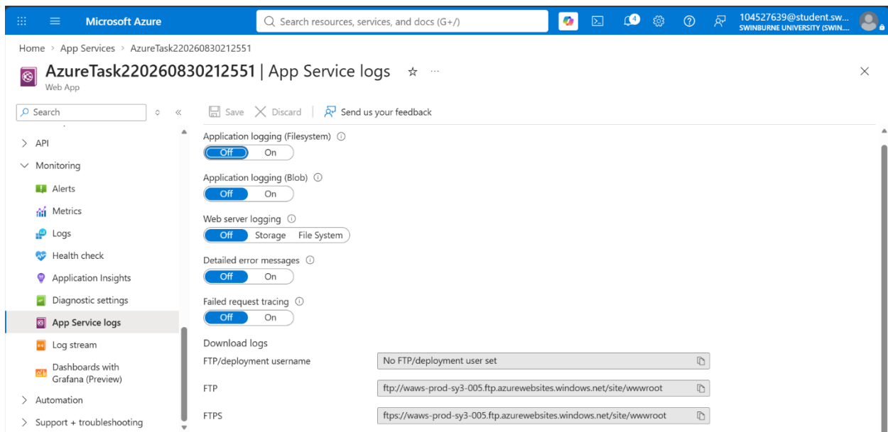
Figure 19: Configuring Azure App Service logging for application and web server diagnostics.
