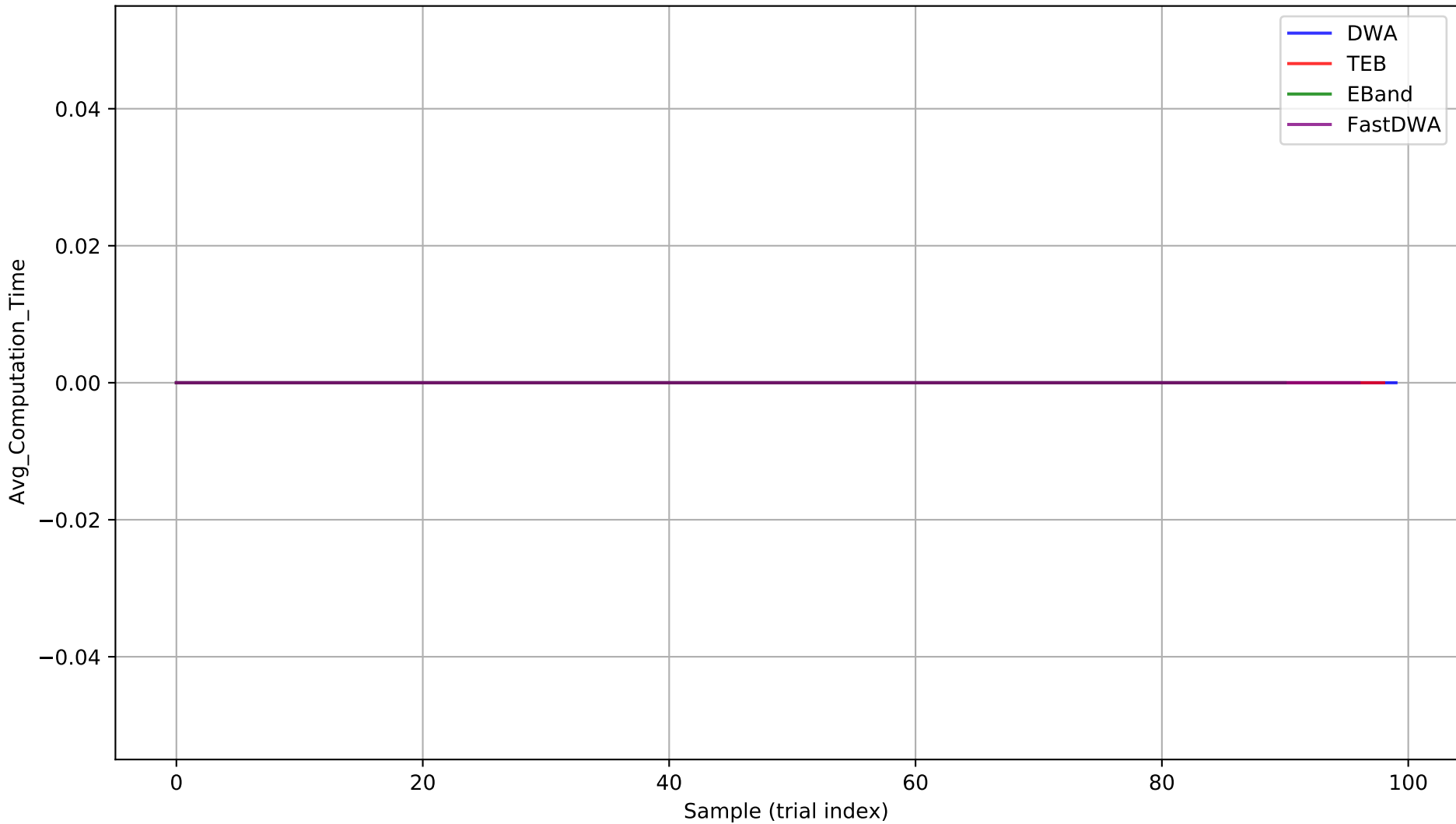
Metric: Avg_Computation_Time
