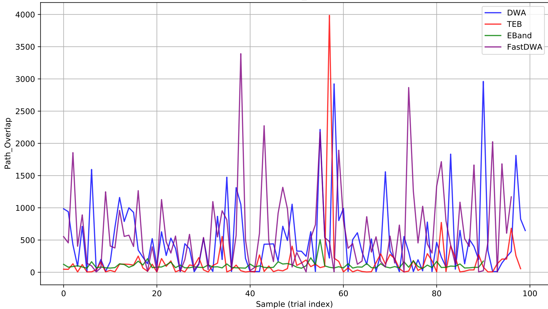
Metric: Path_Overlap
