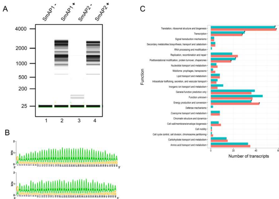
Figure 4. Elevated levels of the SmAPs increase the abundance of RNAs with A-rich tails. (A) Total RNA was isolated from strains PH1-16(pMJ05-SmAP1-His) and PH1-16(pMJ05-SmAP2-His) grown either in the presence of sucrose (–, non-induced) (lanes 1 and 3) or arabinose (+, induced) (lanes 2 and 4). Equal amounts of total RNA were used to isolate adenylated RNA with the Oligotex™ kit. Two microliter of each eluate was analyzed using with the Agilent 2100 Bioanalyzer (Agilent Technologies) and the RNA 6000 Nano Kit (Agilent Technologies). (B) The sequence composition of the A-rich tails obtained after over-production of SmAP1 (top) and SmAP2 (bottom) was determined using WebLogo (51). Only 3' ends of the adaptor clipped reads, which do not map to the reference genome and which showed an overhang of longer than 15 nt were used for the analyzes. Only sites present in both replicates that are supported by at least five independent reads were analyzed. (C) Functional categorization of tailed RNAs. Functions, which are significant enriched (Fisher's exact test; \alpha = 0.05 ) are marked with an asterisk. Genes are annotated according to (54).
