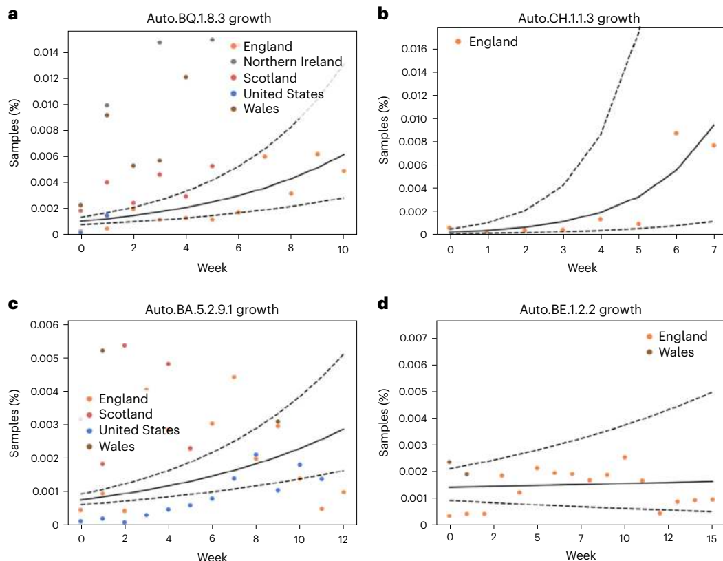
Fig. 2 | Exponential growth modelling. a–d , The four plots describe some of the lineage annotations produced by our method based on the public SARS-CoV-2 data. The solid black line is the median estimated growth trajectory, while the dashed lines represent the trajectories that would result from the lower and upper bounds of the 95% credible interval of the growth rate. The x-axis shows the weeks since first detection in each country. a , Growth trend of a lineage
