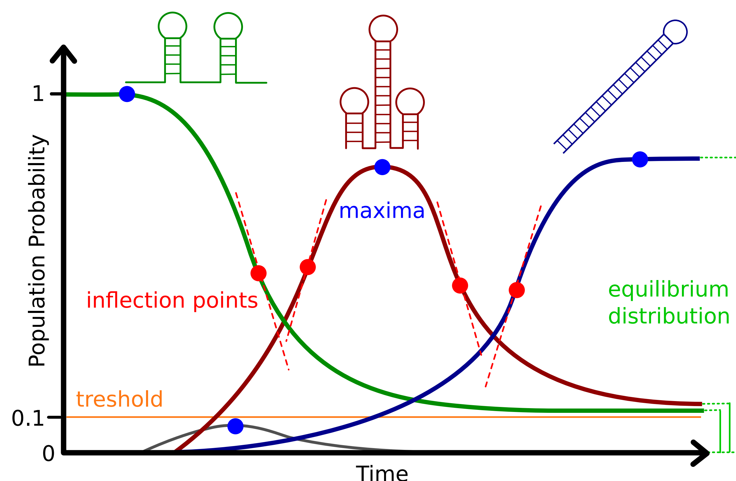
Fig. 2: The kinetics of the system need to be calculated during the iterative process of optimising the sequence. The obtained curves are then evaluated using curve sketching and numerical integration.
