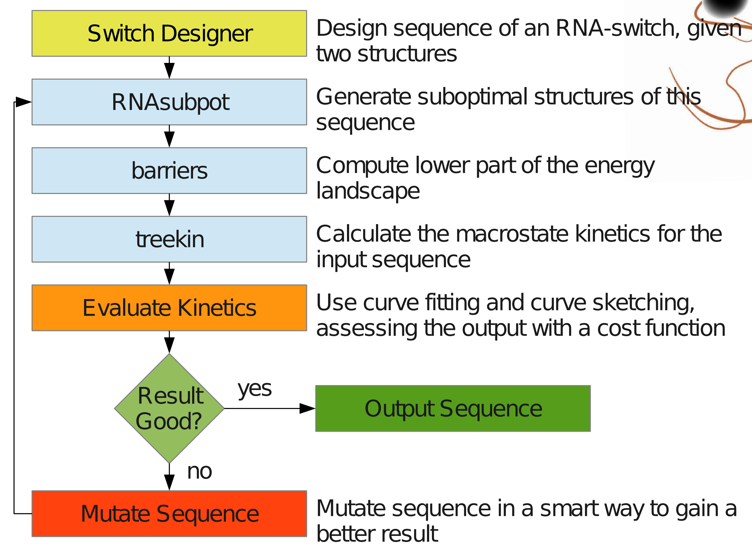
Fig. 3: The design pipeline consists of three parts. As a start-sequence we use a bistable RNA molecule and optimise it to become tri- or multistable. The obtained sequence is then evaluated by a cost function after calculating the Energy Landscape and the Kinetics of the system. If the result is good enough it will be exposed to the user, otherwise it will be mutated according to the graph coloring method and resubmitted to the process.
