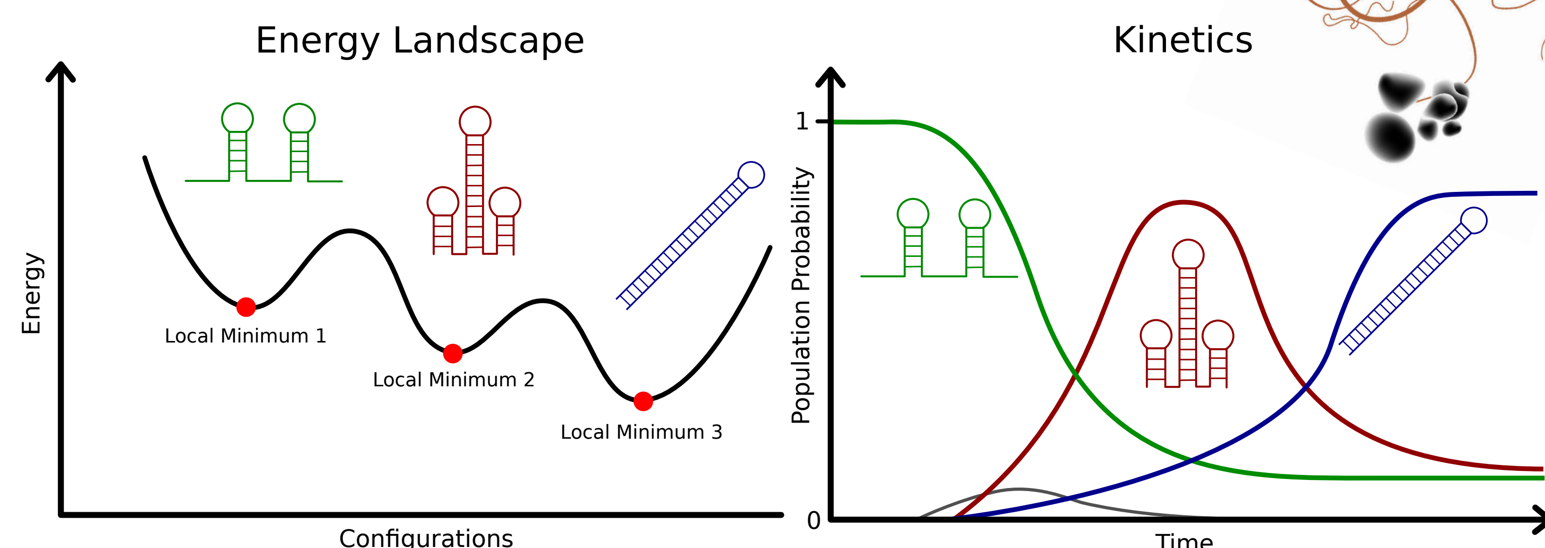
Fig. 4: The resulting sequence folds into more than two given secondary structures and strictly follows predefined conformational and kinetic properties. Upcoming metastable structures should be avoided while the RNA molecule folds into the given conformations during time.
