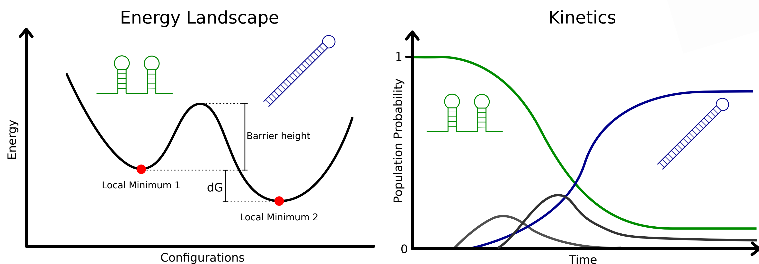
Fig. 1: Schematic representation of the Energy Landscape and the transition between the two states of a bistable RNA switch over time. Notice that other metastable conformations are appearing during the transition.
