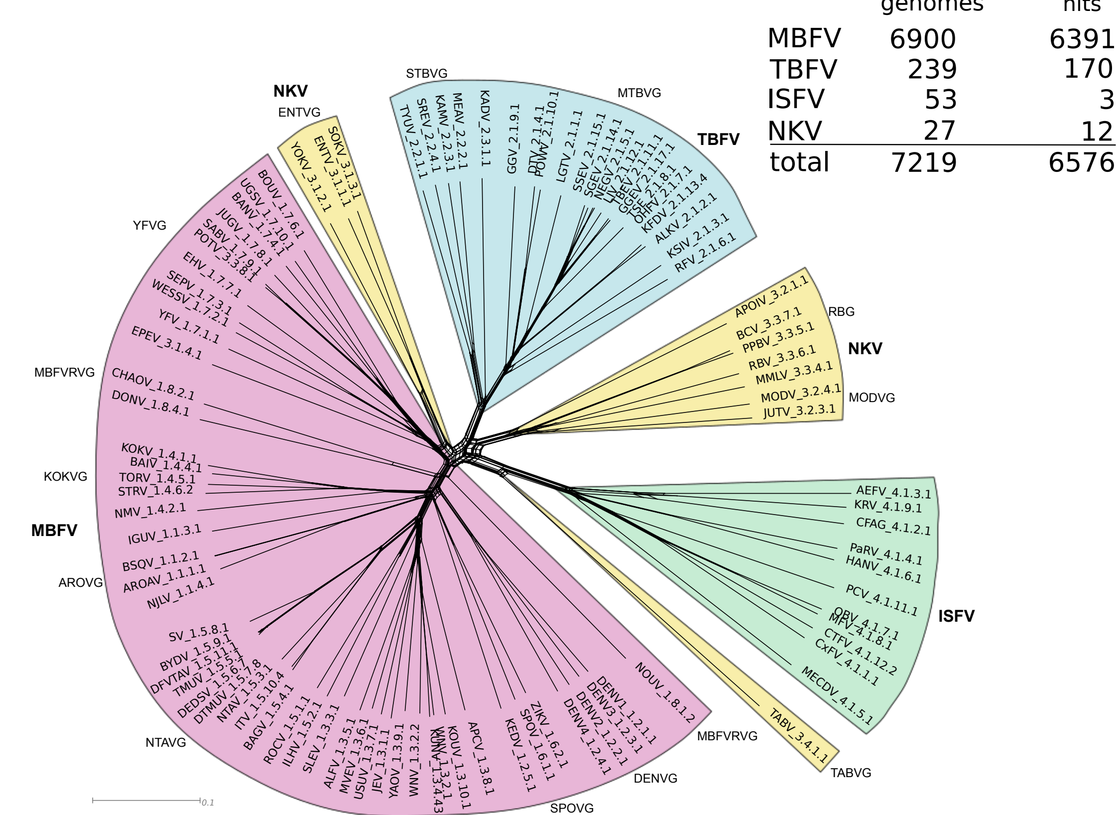
Fig 4. Phylogenetic network of 95 different FV species. Neighbor net computed from ClustalO multiple sequence alignment of annotated protein coding regions.
