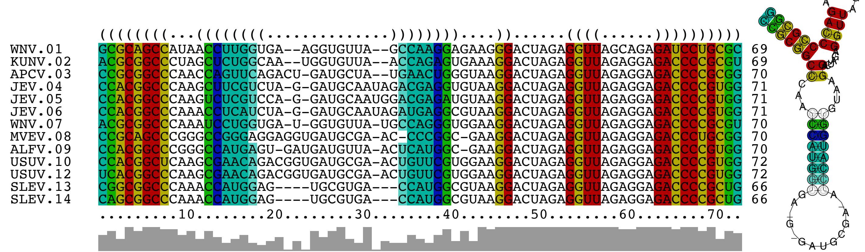
Fig 2. Correlation in a structural alignment of JEVG viruses (left). Paired positions show a high amount of compensatory mutations. Consensus structure (right) computed with RNAalifold [3].
