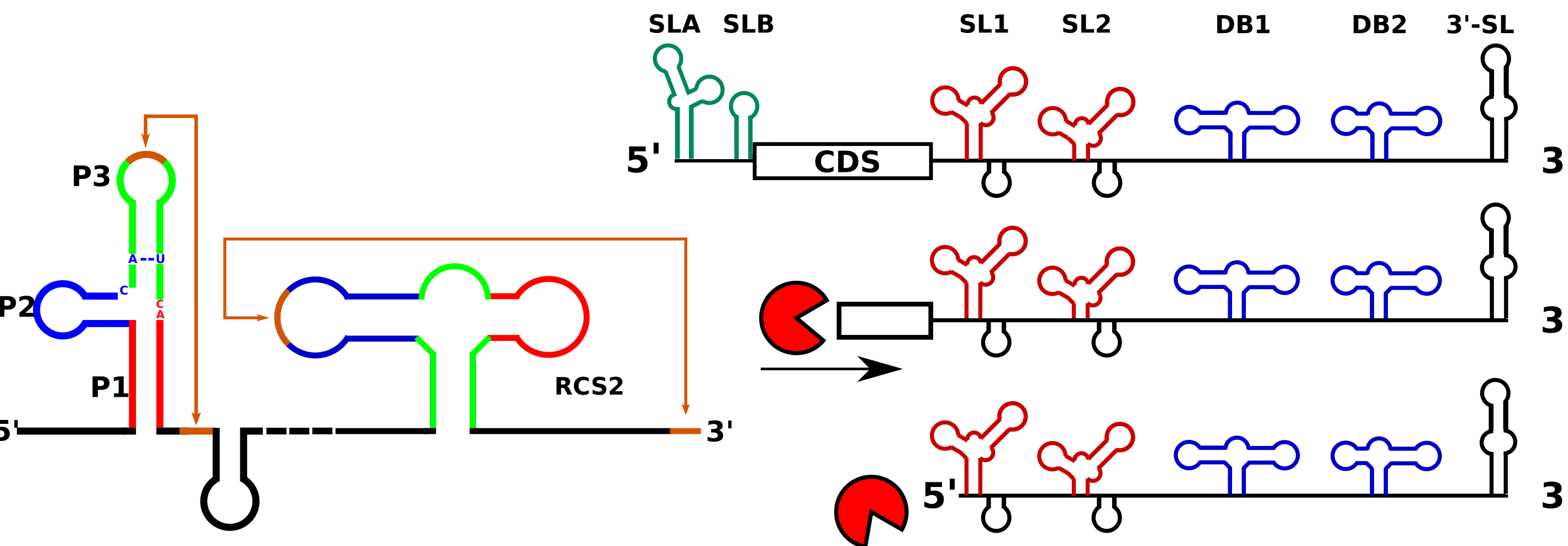
Fig 1. Schematic representation of FV genome organization (top right). Conserved xrRNA elements SL and DB (left) are located in single or tandem within 3'UTRs and efficiently stall host exonuclease Xrn1 (red pac-man). A pseudoknot interaction has been reported for some SL and DB elements (orange, left).
