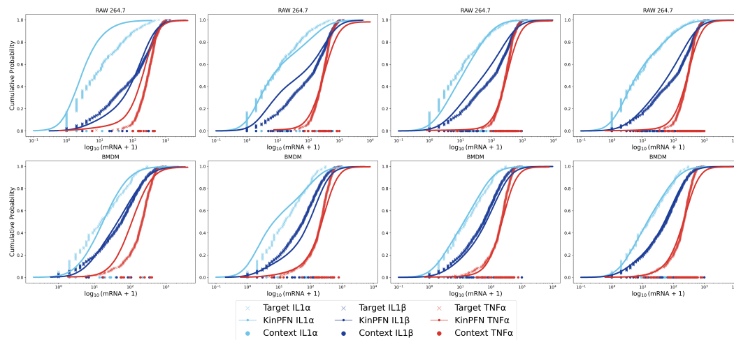
Figure 17: Approximation of mRNA expression of IL-1α , IL-1β and TNF-α in RAW 264.7 and BMDM cells. We plot approximations using only 10, 25, 50 and 75 context data points per gene.
