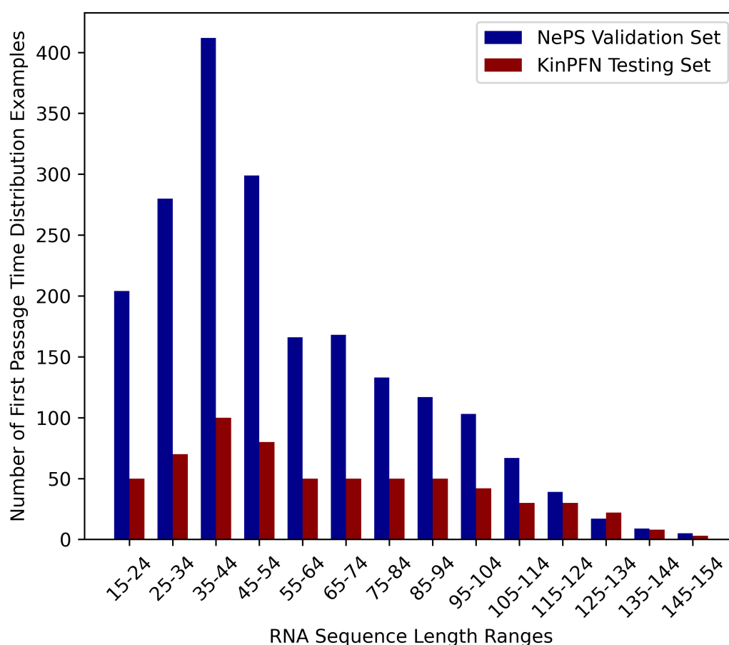
Figure 9: Number of examples by RNA sequence length ranges for the custom validation set used in all NePS (Stoll et al., 2023) i.e., Hyperband (Li et al., 2017) iterations and the custom testing set used for final KinPFN model evaluations (Section 5.1). Both sets are independent of each other with respect to RNA primary sequence and secondary structures.
