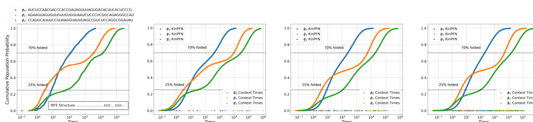
Figure 16: RNA folding efficiency analysis. The first plot from the left shows the ground truth CDFs F(t) for three sequences \phi_0, \phi_1 and \phi_2 , representing the fraction of molecules folded into the MFE conformation over time t . The second, third, and fourth plot displays the KinPFN approximations \hat{F}(t) with ten, 25, and 50 Kinfold times as context.
