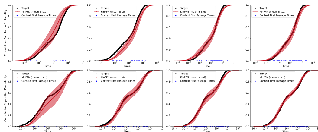
Figure 11: KinPFN first passage time CDF approximations with context times N \in \{10, 25, 50, 75\} (left to right) for a 31 nucleotide long RNA (top) and a 56 nucleotide long RNA (bottom). First passage times were obtained using the kinetic folding algorithm Kfold Dykeman (2015).
