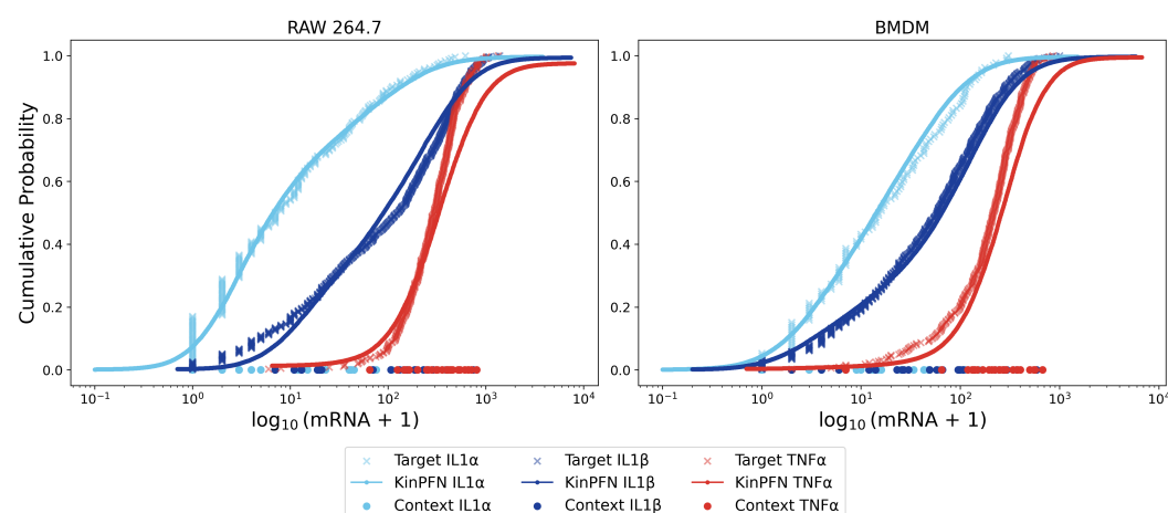
Figure 6: Approximation of mRNA expression of IL-1 \alpha , IL-1 \beta and TNF- \alpha in RAW 264.7 and BMDM cells. We plot approximations using only 25 context data points per gene.
