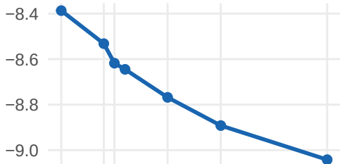
Held-out Likelihood
