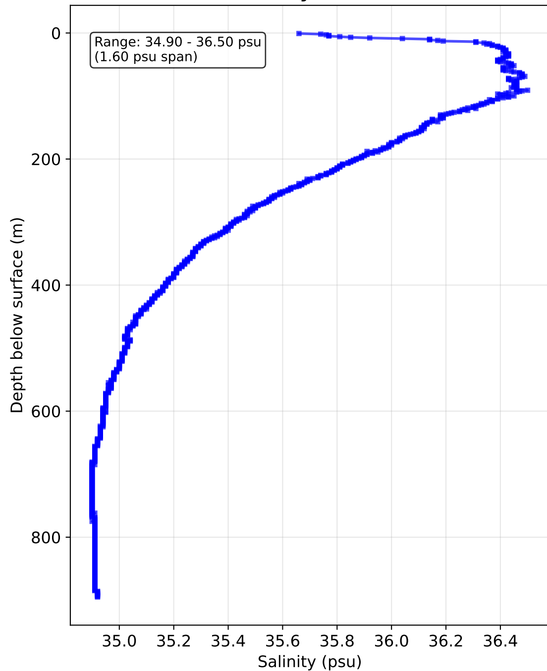
Salinity Profile
