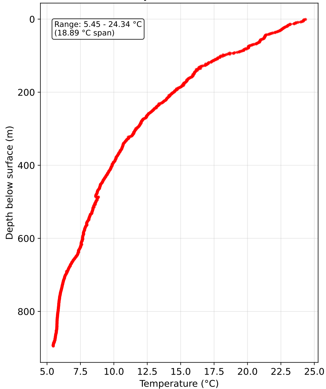
Temperature Profile
