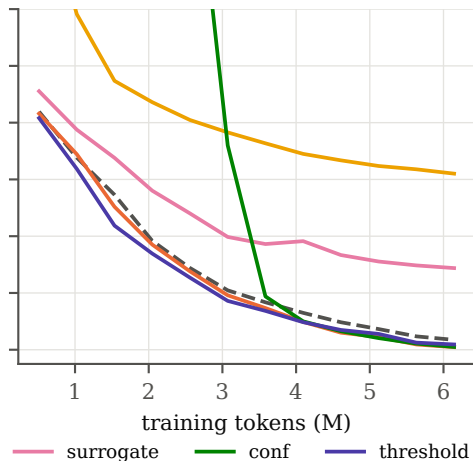
Exp. 2: top-1, raw gate
