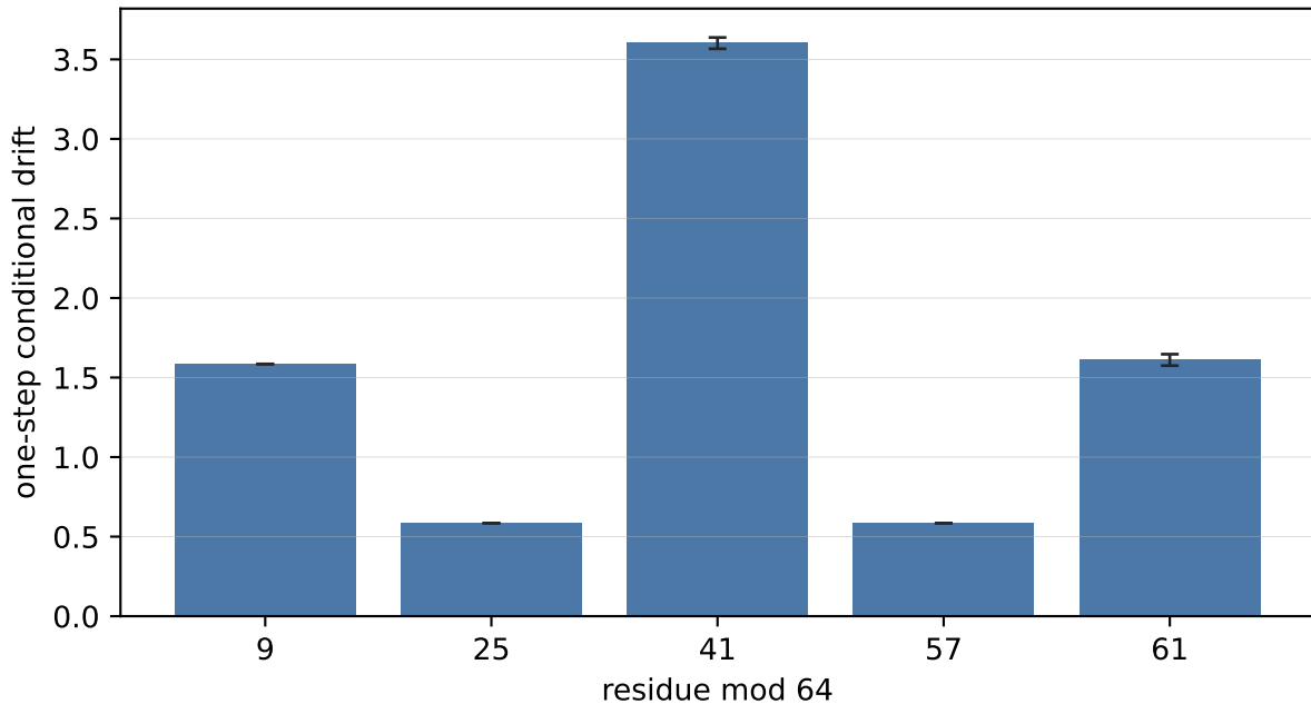
Positive residue obstructions at k=6
