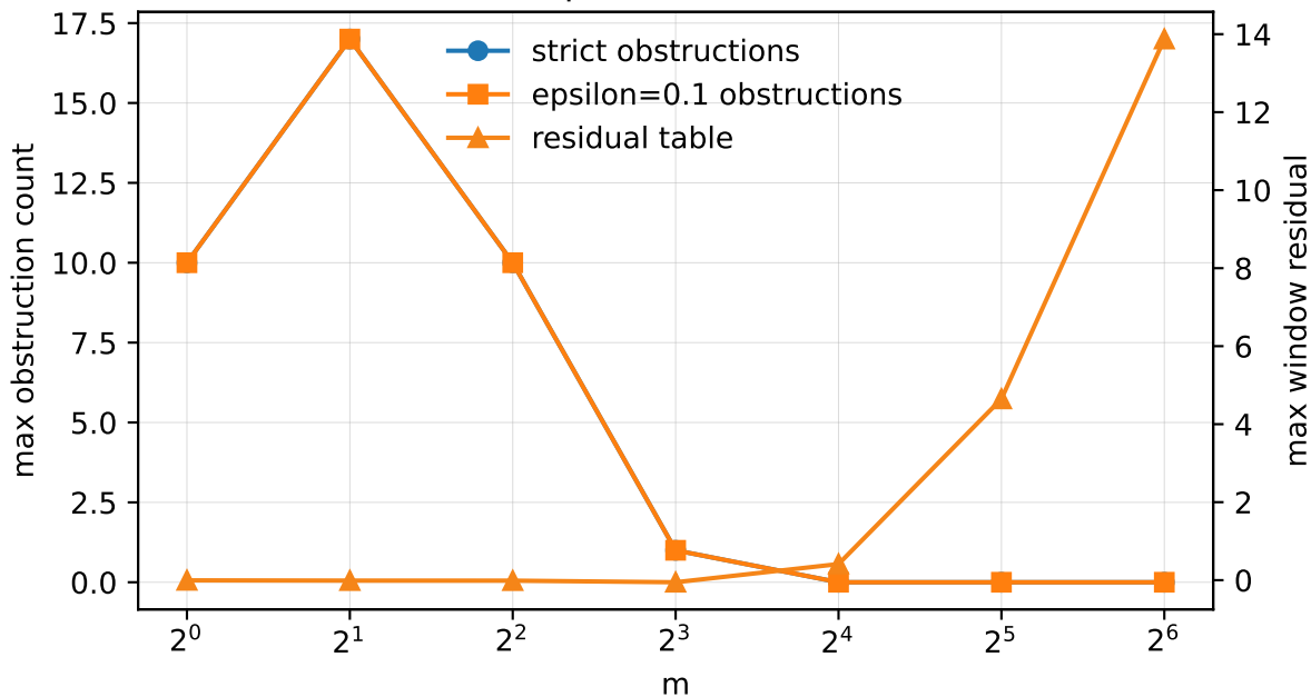
m-step Foster transition
