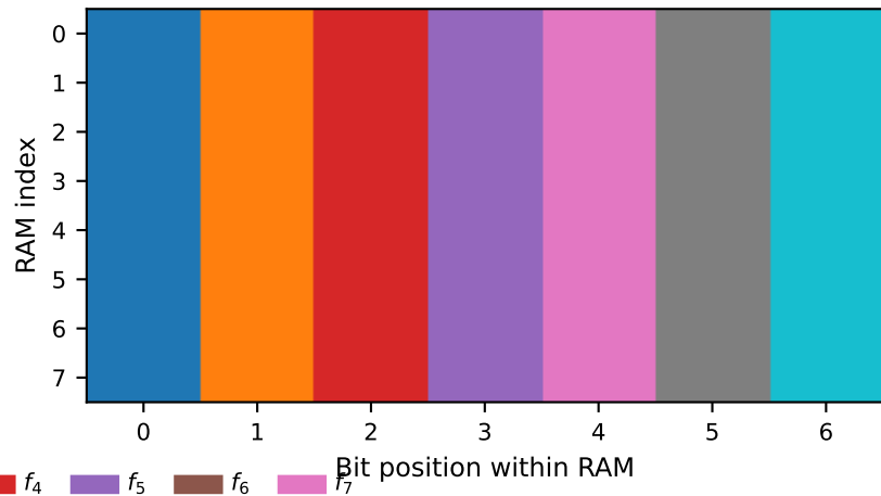
F4RM mapping
