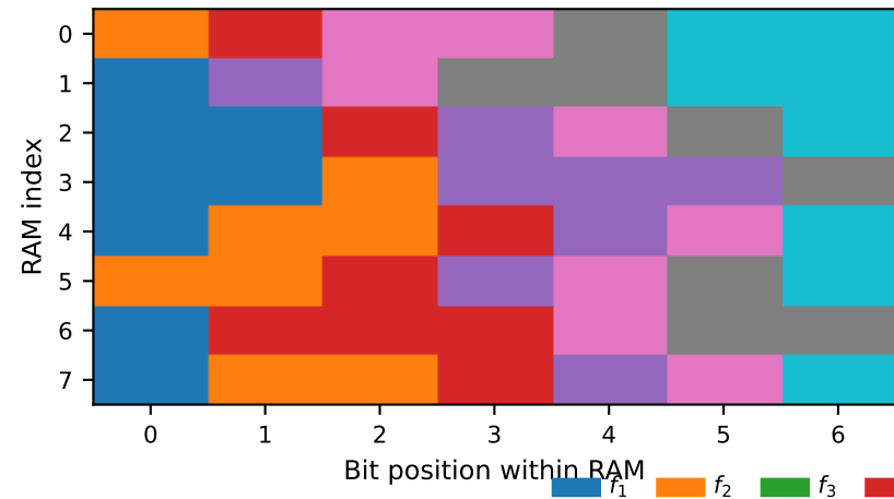
Random mapping
