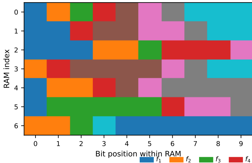
Random mapping
