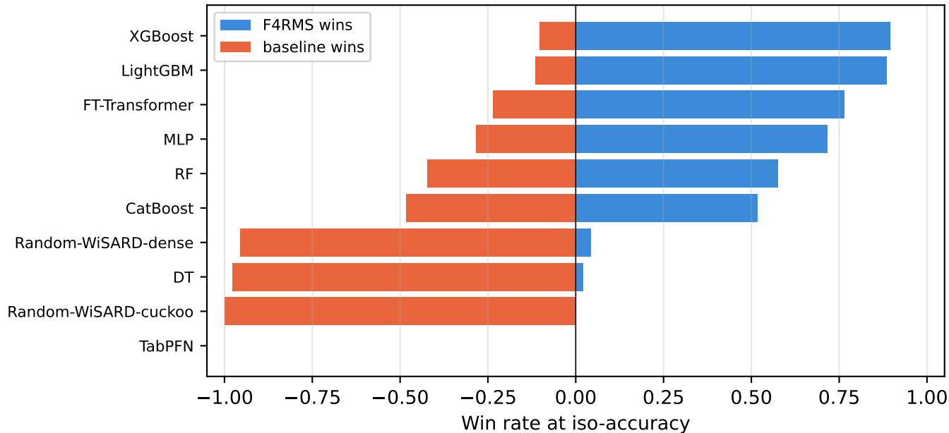
Iso-accuracy: F4RMS vs baselines
