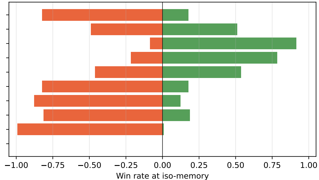
Iso-memory: F4RMS vs baselines
