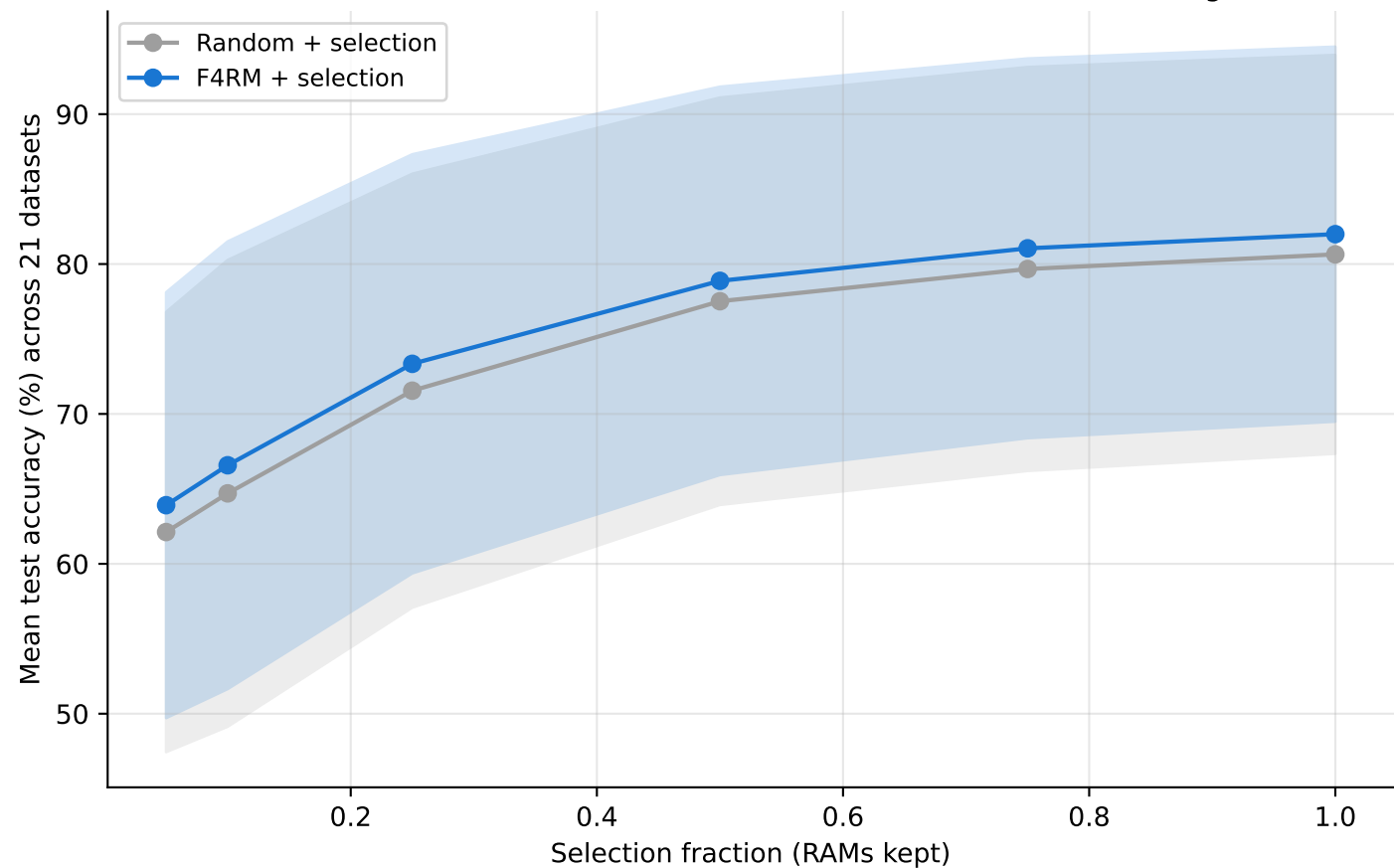
E10: F4RM + selection vs Random + selection (validation scoring)
