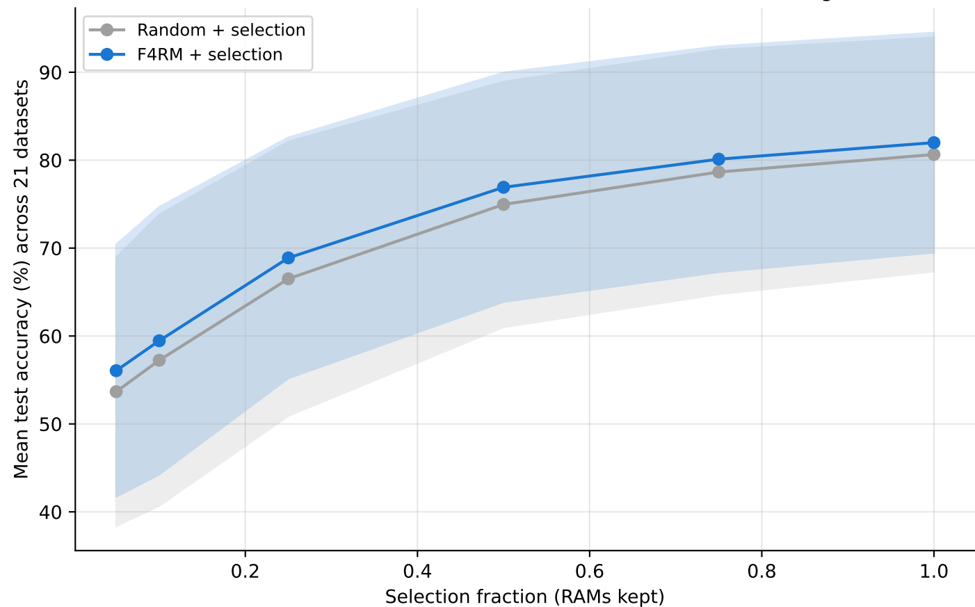
E10: F4RM + selection vs Random + selection (fisher scoring)
