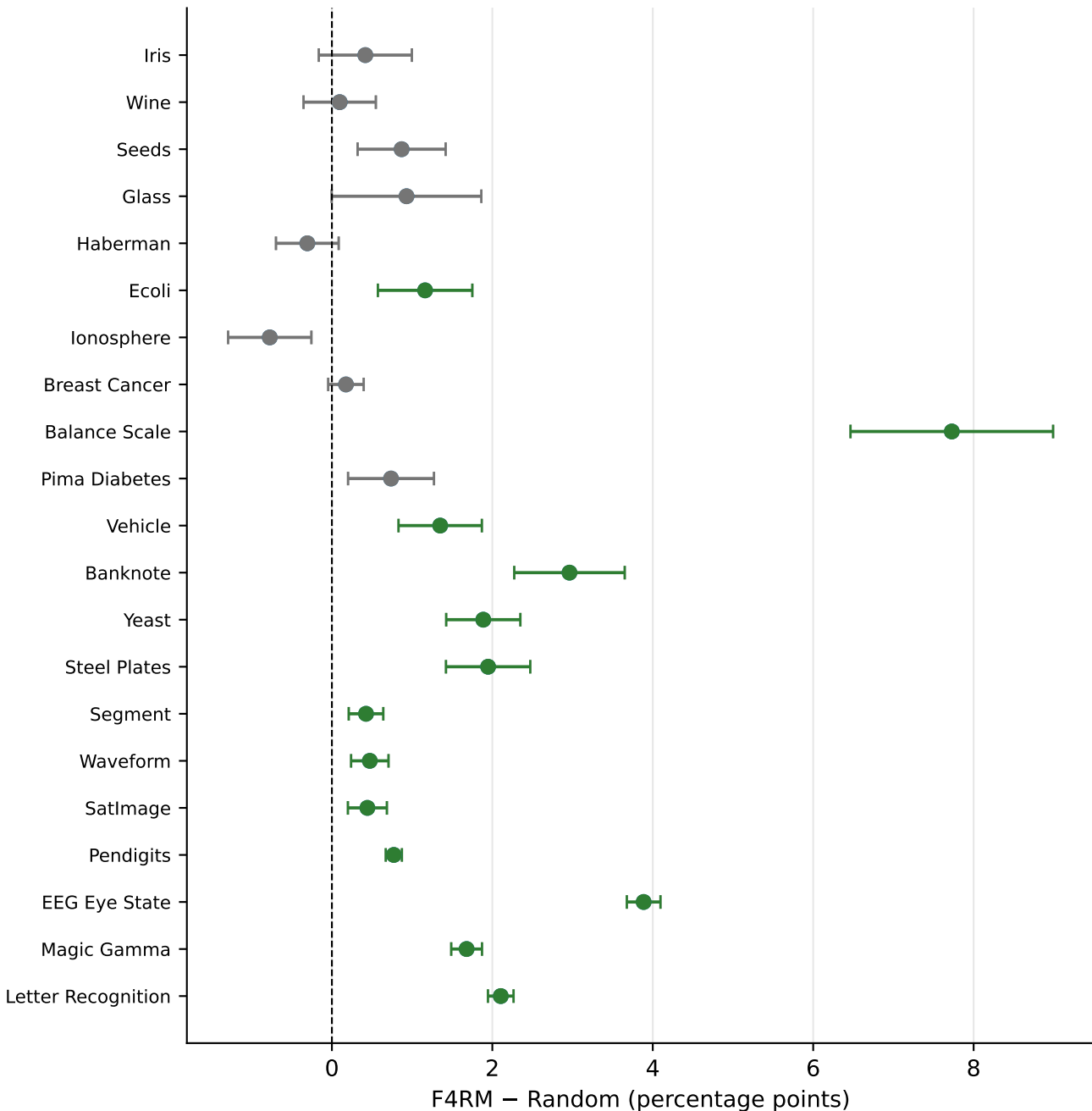
E1: F4RM vs. Random paired delta, 95% CI (200 paired splits)
