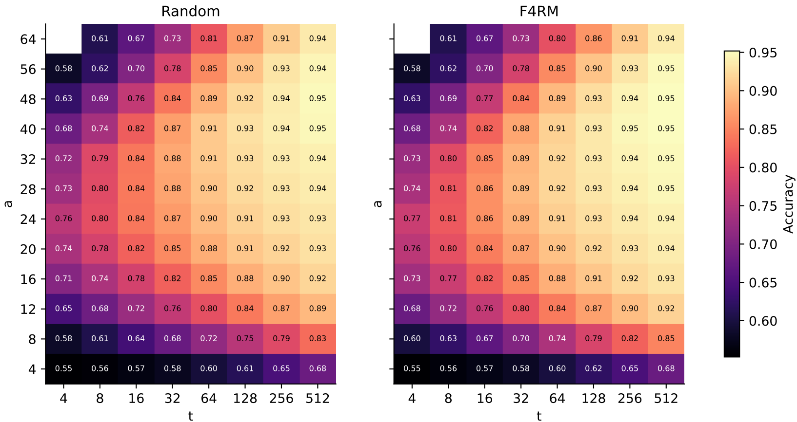
E4: EEG Eye State accuracy heatmap, Random vs. F4RM mapping
