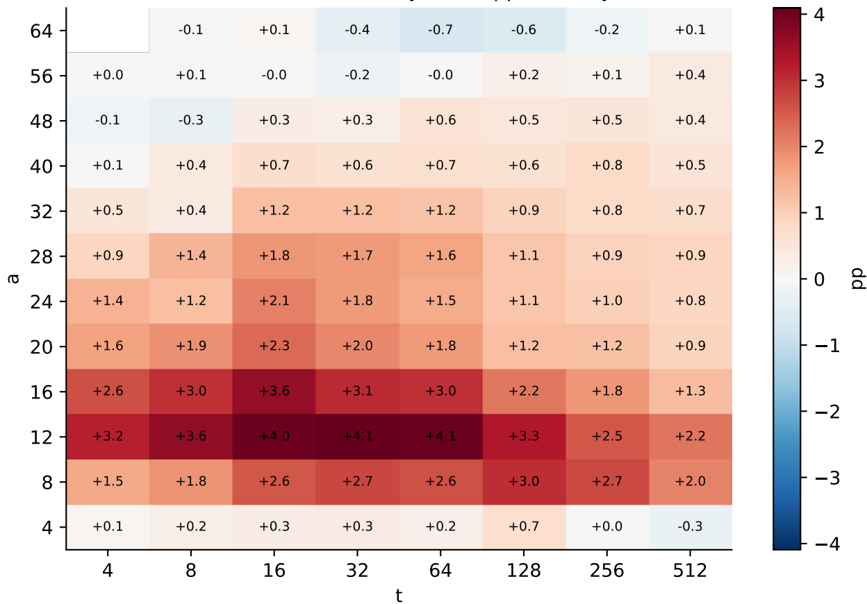
E4: F4RM – Random accuracy delta (pp), EEG Eye State
