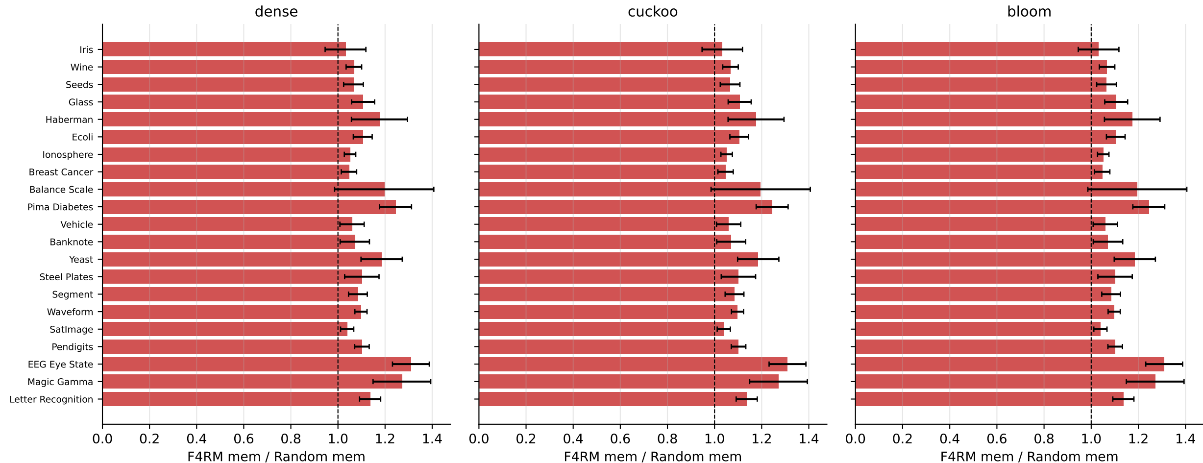
E8: F4RM/Random memory ratio across storage backends (green = F4RM uses less memory; black dashed = parity)
