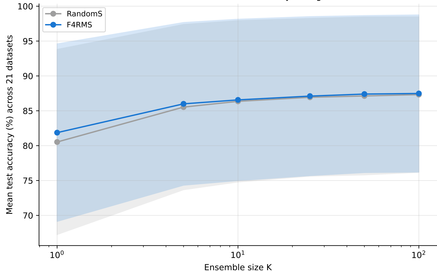
E9a: F4RMS vs RandomS accuracy as K grows
