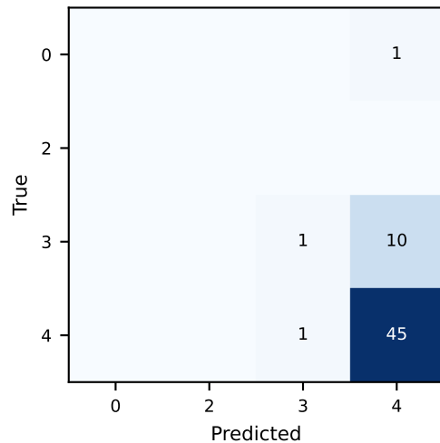
Wave (MobileViT-S)
