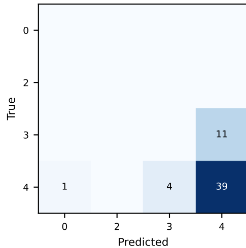
Wave (MobileViT-S)
