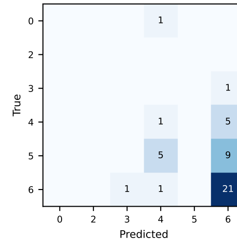
Overlapped Pencils (MobileViT-S)
