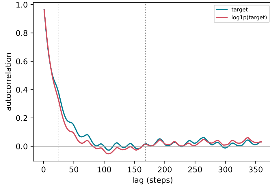
ACF decays within \sim 2 days; weak 24-step bumps
