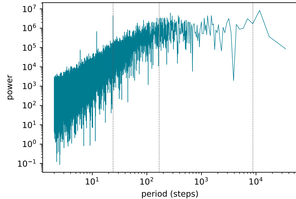
Periodogram, \log_{10}(\text{target})
