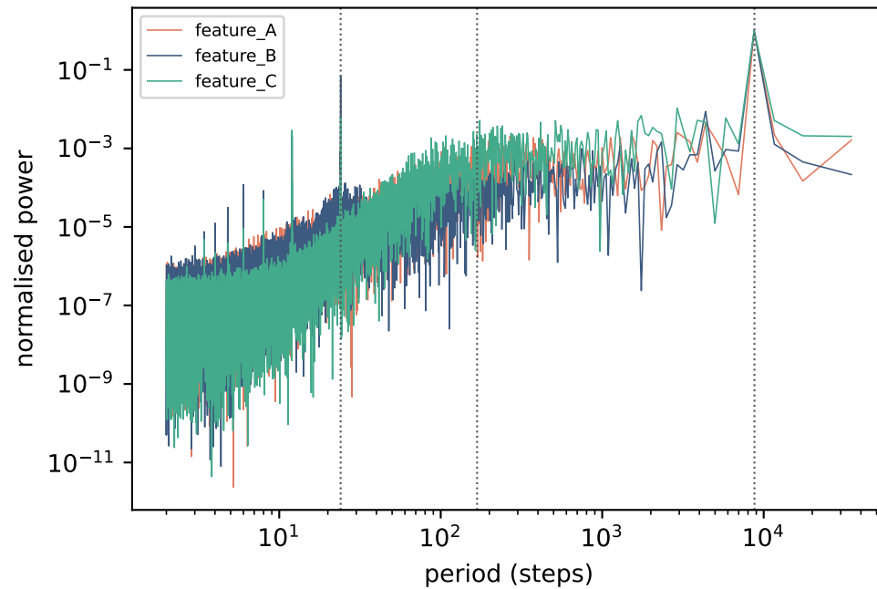
Periodogram, continuous covariates A-C
