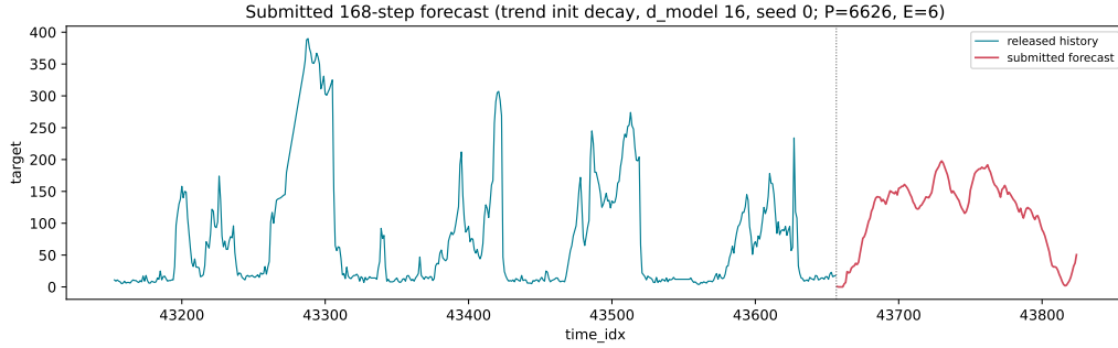
Figure 6: Last three weeks of released history and the submitted 168-step forecast.
