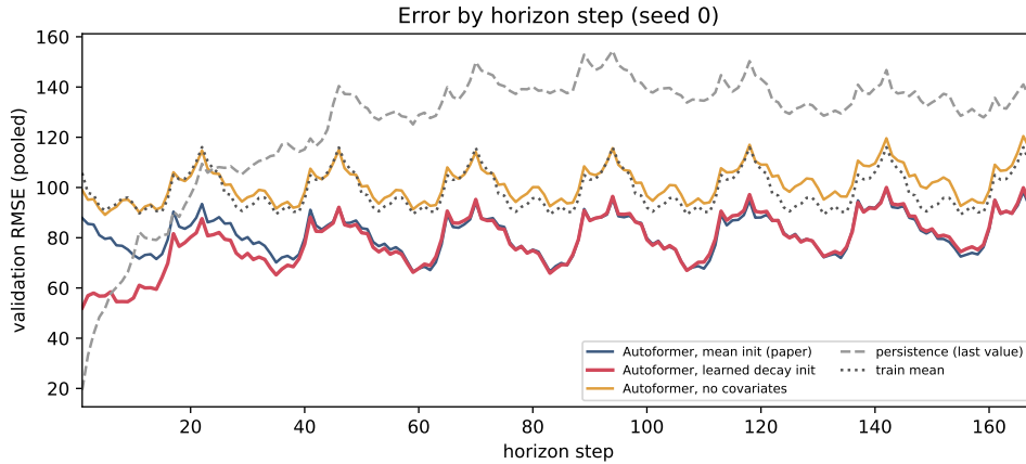
Figure 5: Validation RMSE by horizon step (seed 0). The decay initialisation follows persistence early and the mean-initialised model late.
