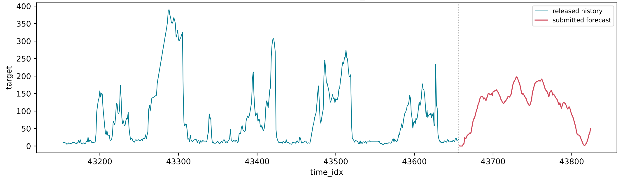
Submitted 168-step forecast (trend init decay, d_model 16, seed 0; P=6626, E=6)
