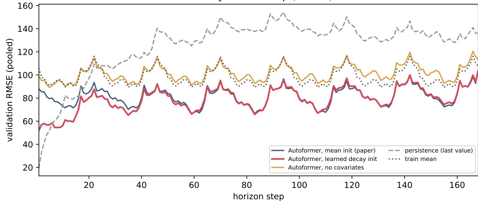
Error by horizon step (seed 0)
